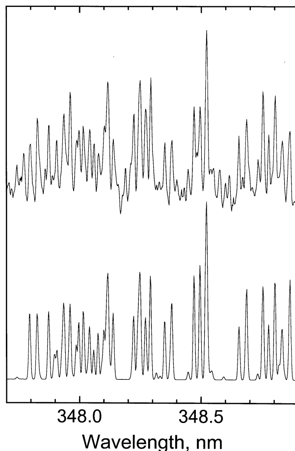
Fig. 6. Comparison of a HIRES spectrum (top) and a DIATOM spectrum (bottom) containing the Herzberg I 6–7 band and the Chamberlain 8–2 band scaled for best fit.
