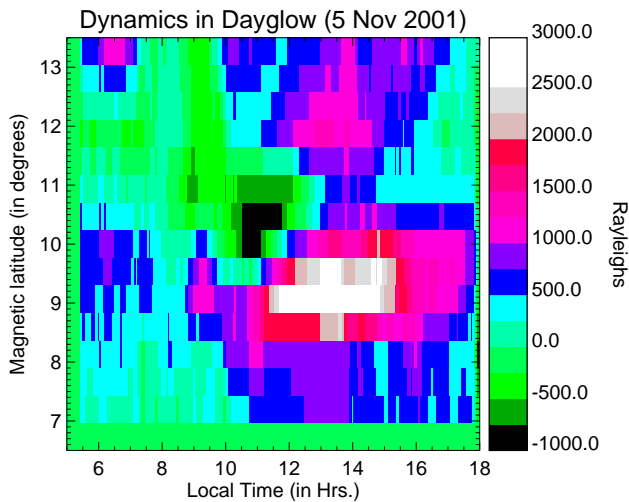
Fig. 6. Two-dimensional plots of the dynamical component in the dayglow for 5 November 2001. The x axis represents the local time and y axis indicates the approximate magnetic latitude in the Southern Hemisphere from where the emissions are assumed to have originated. A constant emission altitude of 230 km has been assumed to estimate the magnetic latitudes. The color scale indicates the brightness variation due to the dynamics of the upper atmosphere in the red line emission region (similar to the bottom panel of Fig. 2). A peak is seen centered at around 13:00 LT at 9° magnetic latitude, which is most likely the response to the EIA development. This weaker development of the EIA as seen in the dayglow emissions, is an indication of weaker equatorial electrodynamics and hence no post-sunset ESF is expected for this night. Compare this day with the 7 November data (Fig. 8) when a stronger EIA development occurred.
