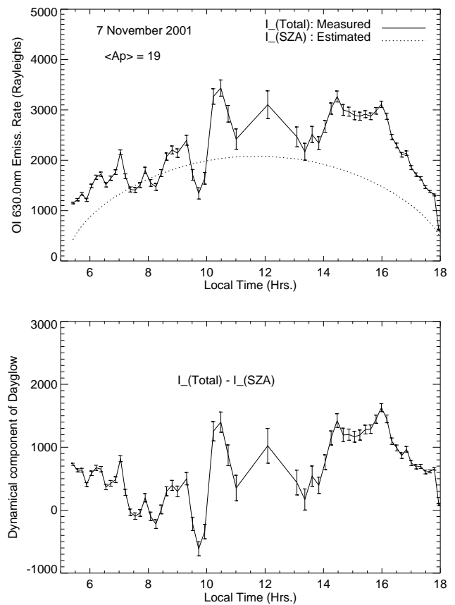
Fig. 4. Same as in Fig. 2 but for 7 November 2001. Notice the periodicities of small-amplitude oscillations, which seem to increase in time periods from around 30 min in the morning to around 100 min in the evening. Whether such a behavior in wave activity is an aftereffect of severe magnetic storms is currently under investigation, as such an increase in the wave periodicities are not seen on the two previous days.
