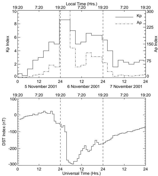
Fig. 1. (Top): K_p and A_p indices for three days 5–7 November 2001. The scales for K_p and A_p are shown on the left and right axes, respectively. K_p index shows a value of more than 4 during the late afternoon hours on 5 November. 6 November is a disturbed day with both K_p and A_p indices of 9 - and 300 respectively. The magnetic disturbance effect is not seen over low latitudes on 5 and 7 November, as can be seen by the low A_p indices on these days. (Bottom): D_{st} variation for the three days under study is shown. The vertical dashed line in both the panels show the 00:00 UT time for the 6 and 7 November data. Storm sudden commencement occurred in the early hours of 6 November and the D_{st} reached a value of -300 nT, indicating a severe storm occurrence. Local time is indicated in the topside of the plot.
