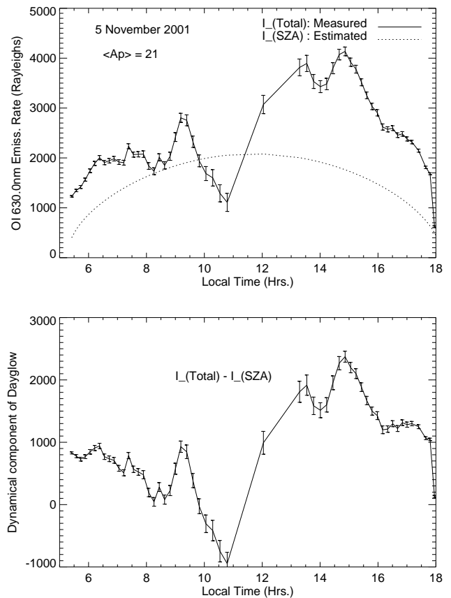
Fig. 2. (Top): Zenith column-integrated OI 630.0 nm dayglow emission rate from Carmen Alto (solid line) and the solar zenith angle (dotted) contribution for 5 November 2001 are depicted along with \pm 1\sigma error bars. The x and y axes represent the local time and the column-integrated emission rate in Rayleighs. The SZA dependent dayglow contribution is obtained by assuming a (\cos)^{0.5} behavior for this variation with SZA and normalizing it with the measured dayglow emissions at around 07:30 LT. The value of the averaged A_p index for the day is shown on top left. (Bottom): Difference between the total column-integrated dayglow emissions and SZA component of the dayglow. This represents the dynamical component in the optical emissions. The negative values represent the “trough-like” features of the wave features. Attention should be paid mainly to the amplitudes of the wave features and not to the negative or positive values alone. A monotonic increase is seen towards afternoon, which is a response of the EIA development.
