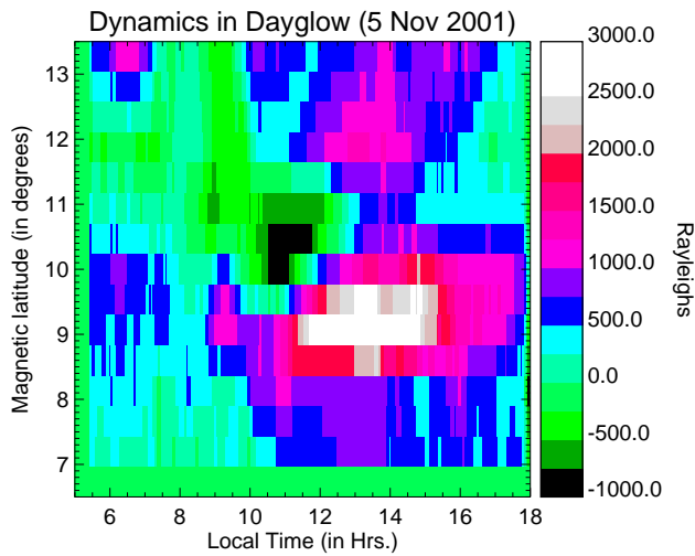
Fig. 6. Two-dimensional plots of the dynamical component in the dayglow for 5 November 2001. The x axis represents the local time and y axis indicates the approximate magnetic latitude in the Southern Hemisphere from where the emissions are assumed to have originated. A constant emission altitude of 230 km has been assumed to estimate the magnetic latitudes. The color scale indicates the brightness variation due to the dynamics of the upper atmosphere in the red line emission region (similar to the bottom panel of Fig. 2). A peak is seen centered at around 13:00 LT at 9° magnetic latitude, which is most likely the response to the EIA development. This weaker development of the EIA as seen in the dayglow emissions, is an indication of weaker equatorial electrodynamics and hence no post-sunset ESF is expected for this night. Compare this day with the 7 November data (Fig. 8) when a stronger EIA development occurred.
