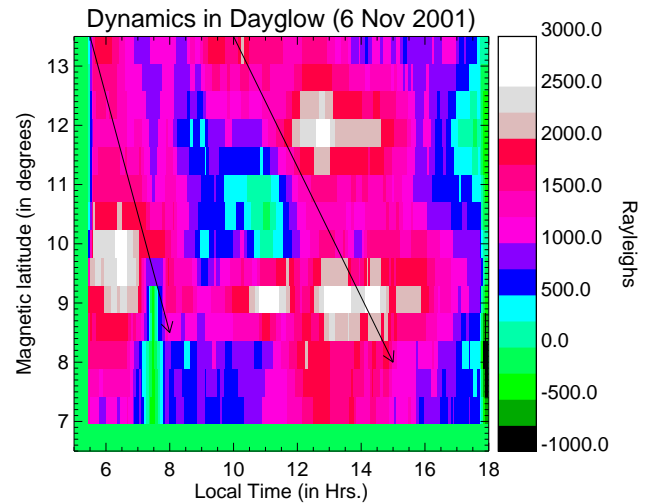
Fig. 7. Same as in Fig. 6 but for 6 November 2001. Notice the sharp rise in the emissions during the morning hours (05:30–08:30 LT), which are 4–5 times larger than the emissions of dynamical component on quiet days, as can be seen in Figs. 5, 6 and 8. The time duration of morning rise is larger in 9°–13.5° magnetic latitudes compared with the duration of increase in 7°–9° magnetic latitudes. Emission enhancements are also seen around 12° and 9° magnetic latitudes at 12:30 LT and 13:30 LT, respectively, most likely indicating propagation of neutral species from high to low latitudes. The arrow indicates a possible direction of the phase propagation of the neutral species from high to low latitudes. The contribution of the dynamical component is largest on this day compared with the quiet days shown in Figs. 6 and 8, possibly due to the presence of comparatively larger neutral densities that are redistributed by the magnetic storm effects.
