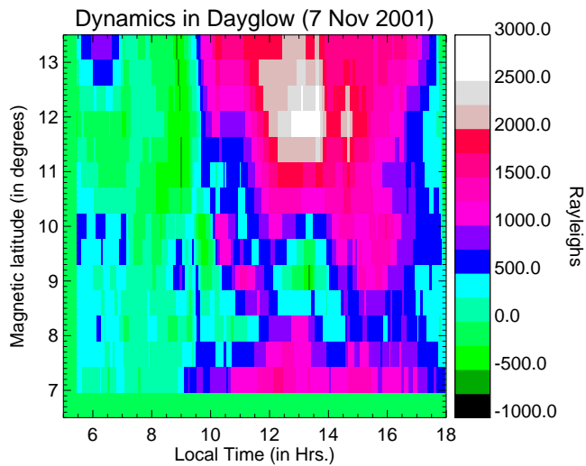
Fig. 8. Same as in Fig. 6 but for 7 November 2001. Notice the strong emissions at around 12^{\circ} – 13^{\circ} magnetic latitude at 13:00 LT. This represents the optical signature of the development of the EIA in the daytime. This day shows relatively stronger EIA development compared with 5 November (see Fig. 6). Such strong EIA developments are conducive for post-sunset ESF occurrence. Jicamarca digisonde data confirmed the post-sunset ESF occurrence on this night. Enhanced 630.0 nm emissions in the afternoon may prove to be the crucial precursors to the post-sunset ESF occurrence.
