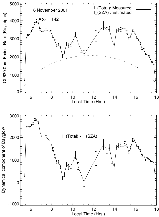
Fig. 3. Same as in Fig. 2 but for 6 November 2001. Notice the rise in emissions in the morning above the dotted line (SZA variation), which is approximately equal to the typical afternoon peak emissions and a factor of 2–3 increase when compared with the morning quiet time emissions (see Fig. 5). The SZA variation used for this day is the same as the one used for all three days. The increase in emissions in the dynamical component in the morning 05:30–08:30 LT (bottom panel) is 4–5 times larger than the typical dynamical variations on a quiet day (see Fig. 5). This brightening is interpreted to be due to the changes in neutral composition over low latitudes. These changes are brought about by neutral winds from high latitudes and TAD triggered by the magnetic storm.
