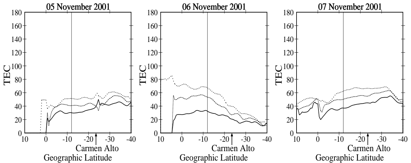
Fig. 10. Total electron content ( \times 10^6 electrons \text{cm}^{-2} ) along American longitude sector, derived from the GPS phase fluctuations for 5–7 November 2001, at 06:00 LT (solid line), 07:00 LT (middle line) and 08:00 LT (dotted line). During this time period, enhancements were observed in the dayglow emissions on 6 November (see Fig. 7). Magnetic equator is shown as a vertical line. Carmen Alto is located at approximately 23.16^\circ geographic latitude as indicated by an arrow. It can be seen that the TEC on 6 November did not show any increase corresponding to the increase in dayglow emissions. Actually, a factor of 1.5–2 smaller TEC was measured on this day compared with the quiet day, thus indicating no role of electron densities in the observed dayglow emission enhancement. Hence, it is suggested that a possible increase in the neutral densities be responsible for the rise in the observed dayglow emissions on this day. Also, the asymmetric nature of the TEC distribution with respect to latitude on 6 November indicates the presence of strong equatorward winds that bring neutrals from the high latitudes.
