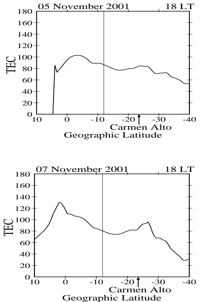
Fig. 9. Total electron content ( \times 10^6 electrons \text{cm}^{-2} ) along American longitude sector (approximately 70^{\circ}\text{W} ), derived from the GPS phase fluctuations at 18:00 LT for 5 November 2001 (top) and 7 November (bottom). Magnetic equator is shown as a vertical line. Carmen Alto is located at approximately 23.16^{\circ} geographic latitude, as indicated by an arrow. It can be seen from the latitudinal distribution of TEC that the development of the EIA on 5 November was weaker compared with 7 November. Compare the 5 November TEC data with the 2-D plot of dayglow emissions in Fig. 6, where no significant emission enhancements are seen poleward of the zenith. On 7 November the latitudinal distribution of TEC shows strong development of the EIA, with a crest poleward of Carmen Alto. Compare this figure with the 2-D plot of the dayglow emissions in Fig. 8, which shows a peak in emissions poleward of zenith on this day. Post-sunset ESF occurred on 7 November and not on 5 November as confirmed by the digisonde data from Jicamarca.
