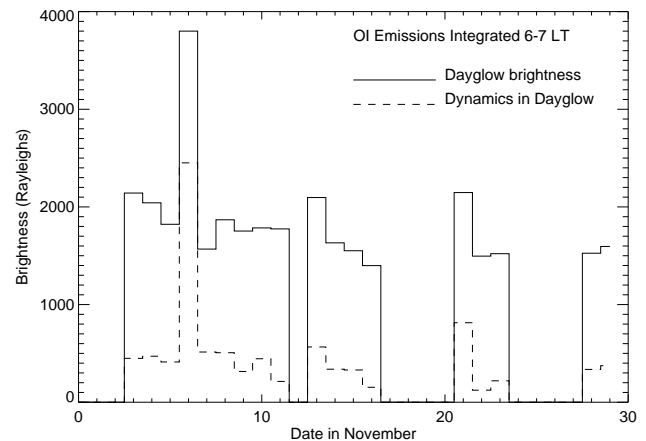
Fig. 5. The average variations of the dayglow brightness (solid line) and the brightness in the dynamical variations (dashed line) during morning hours for 17 days in the month of November. Notice a factor of 2–3 and 4–5 enhancements in the dayglow brightness and in the dynamical component on the disturbed day (6 November when compared with the average variations on the quiet days of the month).
