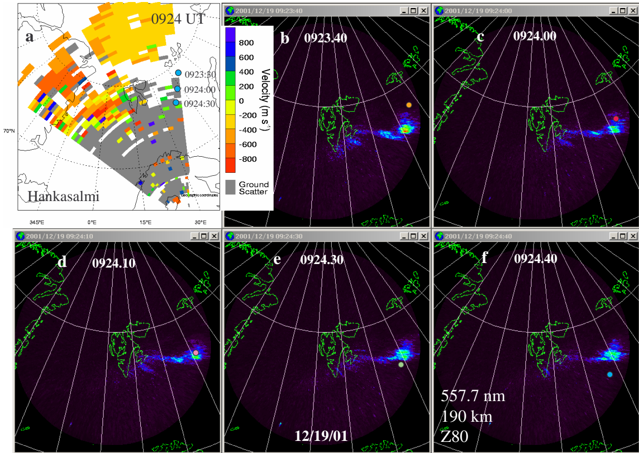
Fig. 15. (b – f) 557.7-nm all-sky images. The images have been extended to 80° zenith angle to cover the mapped positions of DMSP (color-coded circles). Note that in both (c) and (d) the mapped position of DMSP coincides with the optical emissions. SuperDARN line-of-sight velocities from Hankasalmi are displayed in (a), along with the DMSP positions for three times. The large horizontal drift observed by DMSP near 09:24:30 UT is in a region apparently dominated by ground scatter observations.
