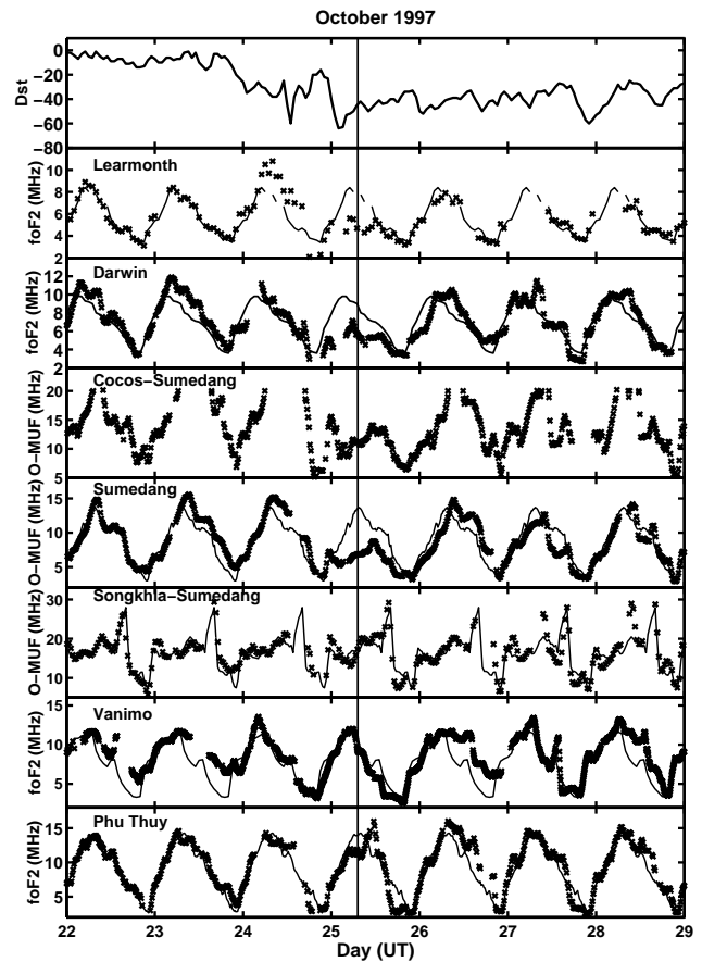
Fig. 5. D_{st} , observed foF2 and maximum oblique-path o-ray frequency values (crosses) and associated medians (line) for the period 22–29 October 1997. The TOPEX/Poseidon pass on the negative ionospheric storm day of 25 October is also shown (vertical line).
