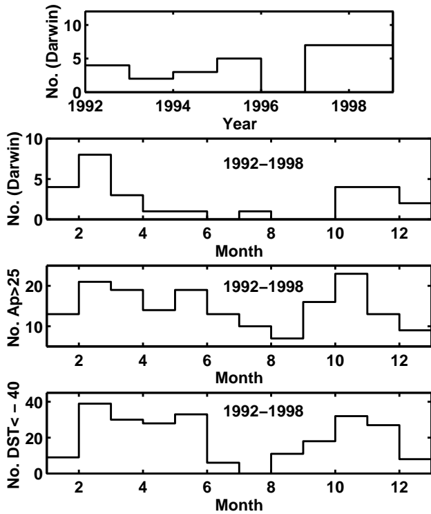
Fig. 2. Ionospheric storm occurrence (Darwin and Townsville) as a function of year and month compared to geomagnetic storm occurrence ( A_p > 25 and D_{st} < -40 ) over the period 1992–1998.
