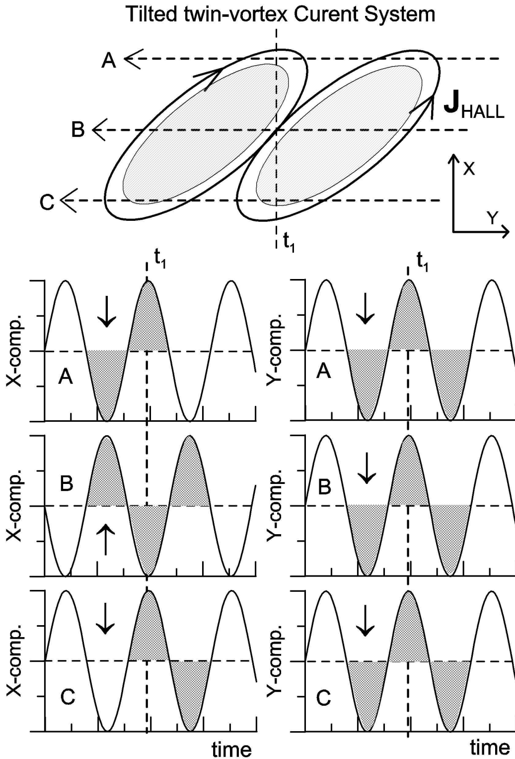
Fig. 15. Tilted twin-vortex current system with opposite polarities of Hall currents, which although naturally moves antisunward above the IMAGE stations, here is considered stationary. Current flow is denoted with an arrow on each vortex structure, while the Sun is located to the left side of this page. The representative ground stations A, B and C are considered to move sunward below the Hall currents. The ground responses, along the three tracks (horizontal-dashed lines) for the three stations, are drawn underneath the vortices. For each track the X and Y magnetometer components are sketched, while it is apparent that at the moment t_1 (vertical-dashed lines) a double phase change of 180^\circ takes place within the latitude range extended from A to C.
