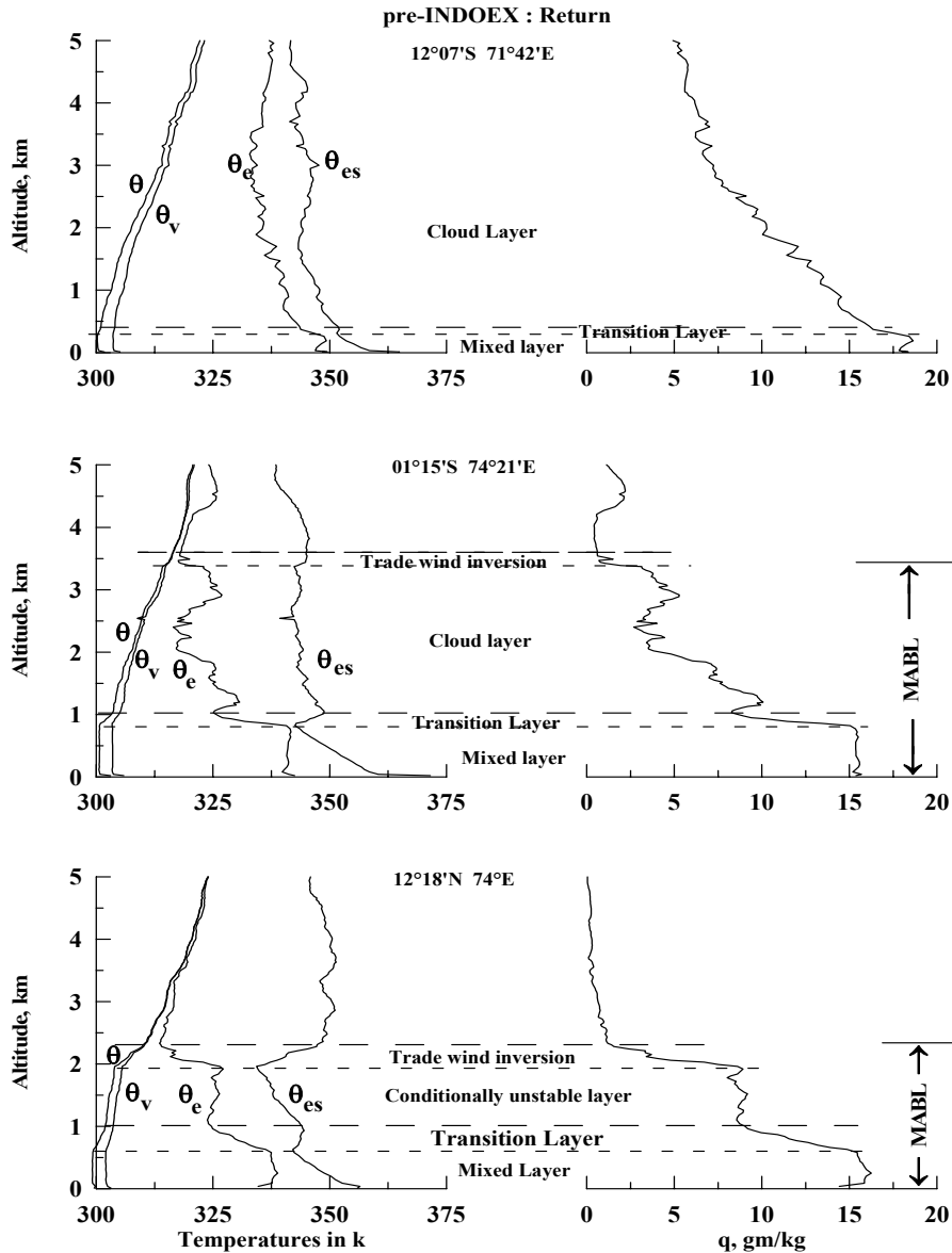
Fig. 3. Altitude profiles of potential temperature ( \theta ), virtual potential temperature ( \theta_v ), equivalent potential temperature ( \theta_e ), saturated equivalent potential temperature ( \theta_{es} ) and mixing ratio ( q ) during the return track of pre-INDOEX.
