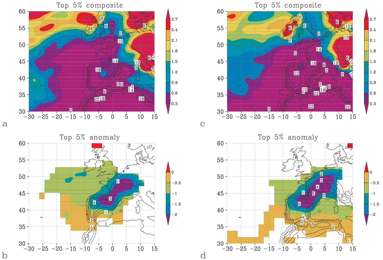
Fig. 8. Composite of precipitation rate in shaded colour (mm/day). For (a) Lisbon and (c) Madrid. Contour lines show the associated temperature range T_{\max} - T_{\min} field ( ^{\circ} C), at 2-m height. The corresponding top 5% anomaly composites, after removing the summer average, are represented in b) Lisbon and d). The precipitation rate anomaly field is represented only in those areas where such an anomaly is significant at the 5% level (or 95% confidence level) computed with a two-tailed t-test.
