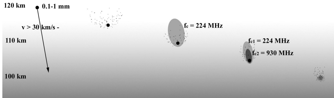
Fig. 1. The meteoroid-atmosphere interaction model based on EISCAT dual frequency observations. The ionized target becomes observable for the EISCAT 224 MHz VHF radar when it reaches the overdense condition at about 110 km. Some six kilometers further down, the effect of further ionization and increased atmospheric density compresses the target to reach the overdense condition, even for the EISCAT 930 MHz UHF radar waves. As the VHF waves do not reach as deep in the target as the UHF, the VHF target is slightly larger than the UHF one. If the geocentric velocity of the meteoroid is 50 km/s, every step in the process occurs with a 0.1-s interval. (Adapted from Pellinen-Wannberg, 2004.)
