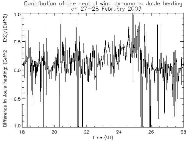
Fig. 7. (c) Percentage contribution of the neutral wind dynamo to Joule heating on the night of 27–28 February 2003.
