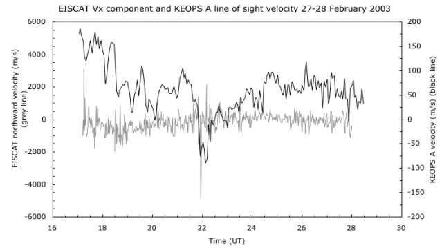
Fig. 3. Comparison of the EISCAT northward component of the field-perpendicular ion velocity (left-hand scale) with the KEOPS FPI line-of-sight thermospheric wind (right-hand scale). The rapid thermospheric response to the ion velocity spike was largely due to a large upwelling caused by Joule heating as shown in Fig. 2b.
