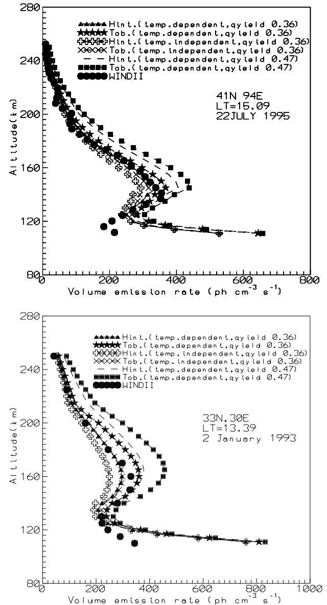
Fig. 3. Same as in Fig. 2 but at different latitudes and local times.
