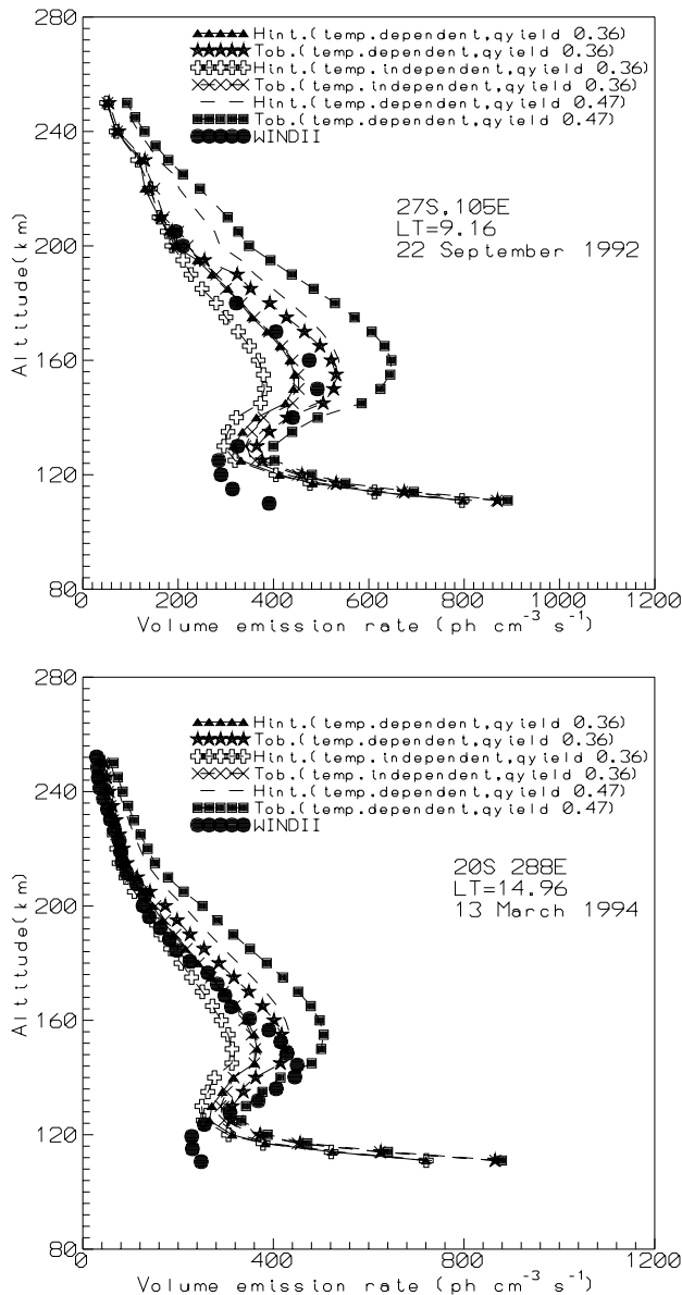
Fig. 2. Comparison between the observed and modelled O(^1S) VER profiles. The darkened triangles and darkened asterisks are for the Hinteregger et al. (1981) and Tobiska (1991) solar EUV flux models with the temperature dependent rate coefficient of reaction N_2(A^3\Sigma_u^+) + O and a quantum yield of 0.36. The plus and the multiplication signs are for the Hinteregger et al. (1981) and Tobiska (1991) solar EUV flux models with the temperature independent rate coefficient of N_2(A^3\Sigma_u^+) + O and a quantum yield of 0.36. The dashed line and the darkened squares are for the Hinteregger et al. (1981) and Tobiska (1991) solar EUV flux models with the temperature dependent rate coefficient of reaction N_2(A^3\Sigma_u^+) + O and a quantum yield of 0.47. The darkened circles are the observed VER from WINDII.
