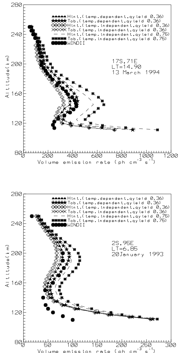
Fig. 1. Comparison between the observed and modelled O( 1 S) VER profiles. The darkened triangles and darkened asterisks are for the Hinteregger et al. (1981) and Tobiska (1991) solar EUV flux models with the temperature dependent rate coefficient of reaction \text{N}_2(\text{A}^3 \sum_u^+) + \text{O} and a quantum yield of 0.36. The plus and the multiplication signs are for the Hinteregger et al. (1981) and Tobiska (1991) solar EUV flux models with the temperature independent rate coefficient of reaction \text{N}_2(\text{A}^3 \sum_u^+) + \text{O} and a quantum yield of 0.36. The dashed line and the darkened squares are for the Hinteregger et al. (1981) and Tobiska (1991) solar EUV flux models with the temperature independent rate coefficient of reaction \text{N}_2(\text{A}^3 \sum_u^+) + \text{O} and a quantum yield of 0.75. The darkened circles are the observed VER from WINDII.
