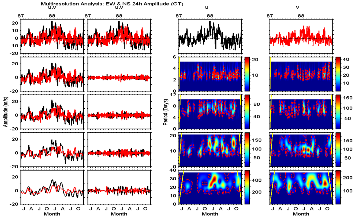
Fig. 3. Analysis of the diurnal tide at Grahamstown: Top row, the original signal A_0 . Rows 2–5, starting from the left, show (1st column) the approximations ( A_m where m is the level), (2nd column) the details ( D_m ), (3rd column) the spectrum of the zonal details and (4th column) the spectrum of the meridional details. The black and red time series lines represent the zonal ( u ) and meridional ( v ) amplitudes, respectively. The scale ( s ) ranges are shown on the left. The units of the colour bars are arbitrary.
