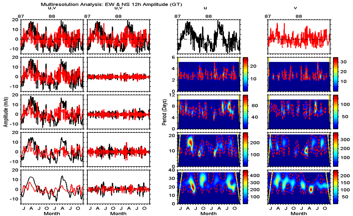
Fig. 4. Analysis of the semidiurnal tide at Grahamstown: Top row, the original signal A_0 . Rows 2–5, starting from the left, show (1st column) the approximations ( A_m where m is the level), (2nd column) the details ( D_m ), (3rd column) the spectrum of the zonal details and (4th column) the spectrum of the meridional details. The black and red time series lines represent the zonal ( u ) and meridional ( v ) amplitudes, respectively. The scale ( s ) ranges are shown on the left. The units of the colour bars are arbitrary.
