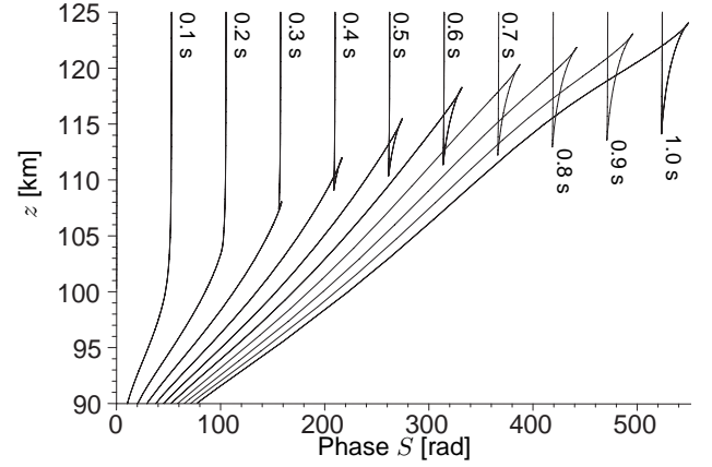
Fig. 4. Phase fronts calculated from the crossing characteristics of Fig. 3 at intervals of 0.1 seconds. This figure shows that some characteristics are associated with multiple phase values: for example S(117 \text{ km}, 0.8 \text{ s}) has values of 395 rad, 415 rad and 425 rad all at the same time and place.
