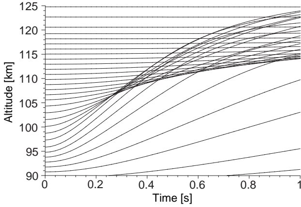
Fig. 3. Characteristic paths z_i(t) obtained by solving the coupled system given by Eqs. (26) and (27) for a 50 mV/m electric field under the assumption of an initially perfectly field-aligned structure.
