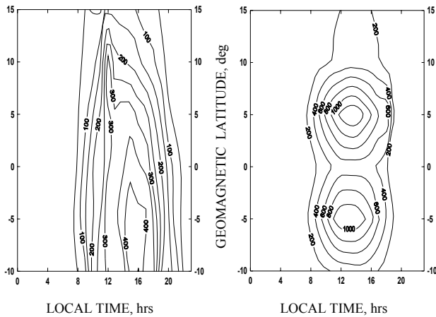
Fig. 8. Latitudinal and local time variation of observed (left panel) and simulated (right panel) O + density at an altitude of \sim 500 km within the geomagnetic latitude range from 10^{\circ} S to 15^{\circ} N during December solstice of low solar activity.
