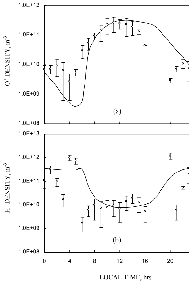
Fig. 6. Local time variation of measured (o) and simulated (—) O^+ density (a) and H^+ density (b) at \sim 500 km altitude in the Indian zone over the geomagnetic equator in the June solstice at solar minimum.
