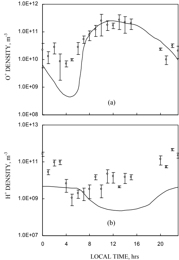
Fig. 7. Same as in Fig. 6 for 10^\circ N geomagnetic latitude.
