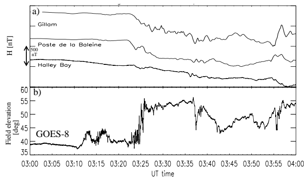
Fig. 4. Magnetic field measurements from different regimes, 24 July 1998. Panel (a) show magnetic H components from the ground stations Halley Bay, Poste de la Baleine and Gillam. Panel (b) show the magnetic field elevation measured in geosynchronous orbit by GOES-8 at 22:20 LT.
