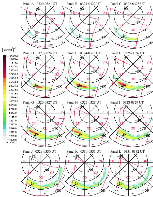
Fig. 3. PIXIE images from the substorm, 24 July 1998, energy range from 2.42–8.82 keV photons. The coordinate system is corrected geomagnetic coordinates (cgm). Local midnight is straight downwards. The ground stations are marked in panel (a) as follows: GIL: Gillam, PBQ: Poste de la Baleine, HBA: Halley Bay, STJ: St. Johns, OTT: Ottawa. Halley Bay is the only Southern Hemisphere station. The magnetic footprint of GOES-8 is marked in black.
