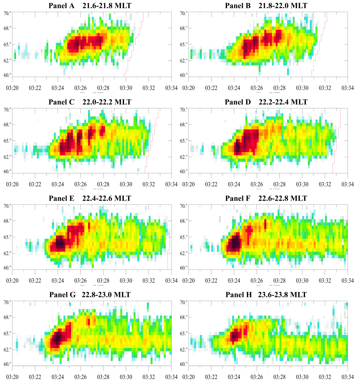
Fig. 6. Keograms for a selection of MLT sectors produced from 2.40–8.82 keV photon measurements by PIXIE. The colour scale is the same as in Fig. 3 and the red line give the border of FOV.
