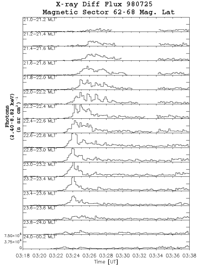
Fig. 5. Time development of X-ray fluxes (2.40–8.82 keV) for several MLT sectors. Fluxes are integrated for 10 s, from 62^{\circ} – 68^{\circ} latitude which covers the whole latitudinal range of the activity.
