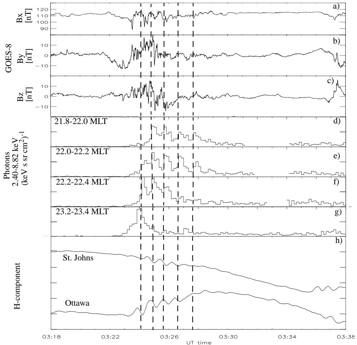
Fig. 7. A composite plot. Panels (a) to (c) show the magnetic field measured by GOES-8 in geosynchronous orbit converted into field-aligned coordinates. The field-aligned direction, B_x , is based on a 5 min average field direction. B_y is in the direction perpendicular to B_x and the spin aligned component B_p which is northward. Panels (d), (e) and (f) are selected MLT sectors from Fig. 5. Panel (g) shows the H component of the two Northern Hemisphere stations Ottawa and St. Johns.
