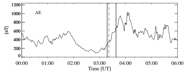
Fig. 1. Provisional AE index from Kyoto for 24 July, 1998. The two vertical lines indicate the time period of PIXIE images, the dashed line gives the time for the substorm onset.
