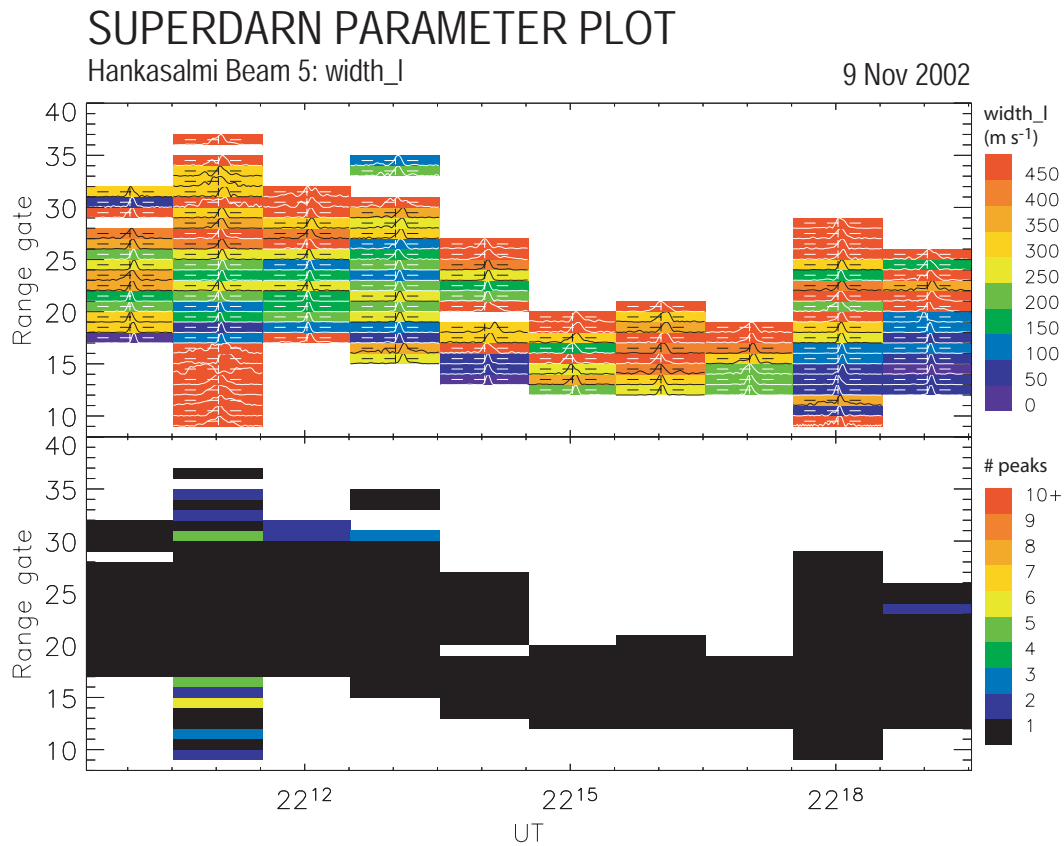
Fig. 3. Top: Spectral width ( width_l ) data from the CUTLASS Finland radar in the same format as Fig. 1 but for the interval 22:09:30–22:19:30 UT. Overlaid on each cell are velocity power spectra derived from the FFT of the radar ACF directly. Vertical lines indicate zero Doppler velocity. Bottom: The number of spectral peaks identified, within 3 dB of the peak spectral power.
