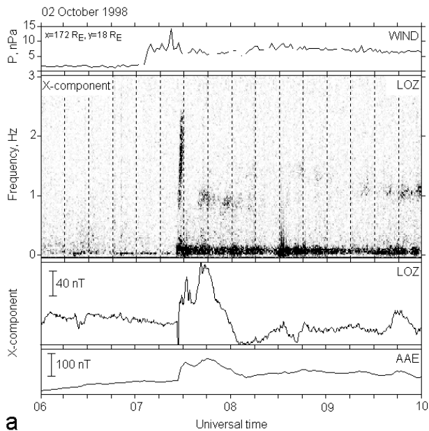
Fig. 4. Excitation of the ULF burst and the increase of the “pearls” carrier frequency during the magnetosphere compression.
