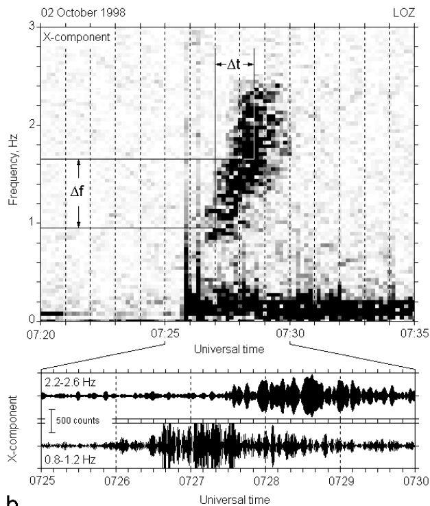
Fig. 3. An example of SB event with the first burst manifested. (a) The same as in Fig. 1. (b) The dispersive characteristics of the first burst (top) and the result of signal filtering in two frequency bands (bottom).
