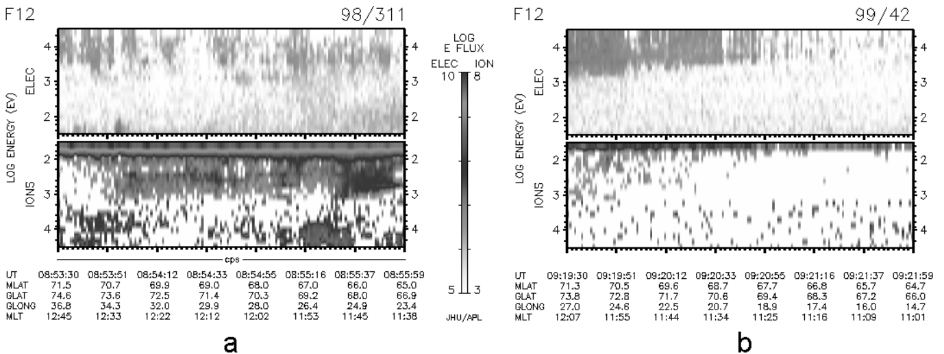
Fig. 7. Comparison of two spectrograms of DMSP F12 for the events (a) and (b) in Fig. 6.
