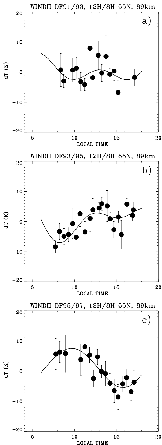
Fig. 1. WINDII temperature semidiurnal and terdiurnal tidal fits at 55^{\circ} N and 89 km height for winter solstice (December, January, and February). The temperature data are two-year composites from 1991 to 1997 fitted simultaneously to 12-h and 8-h tidal harmonics (solid line).
