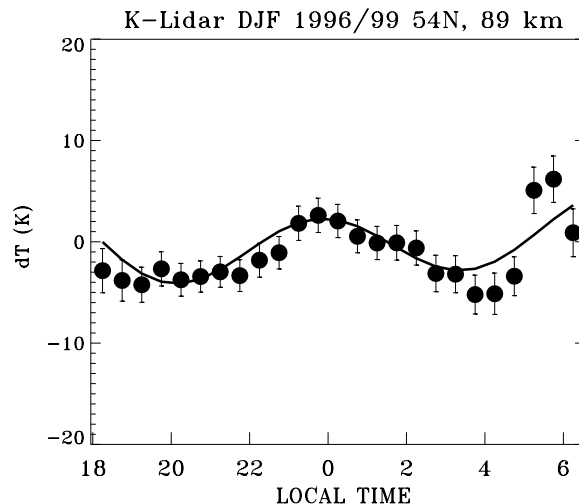
Fig. 2. Potassium lidar temperature semidiurnal and terdiurnal tidal fits at 54^{\circ} N and 89 km height for winter solstice (December, January, and February). The temperature data are three-year composites from 1996 to 1999 fitted simultaneously to 12-h and 8-h tidal harmonics (solid line).
