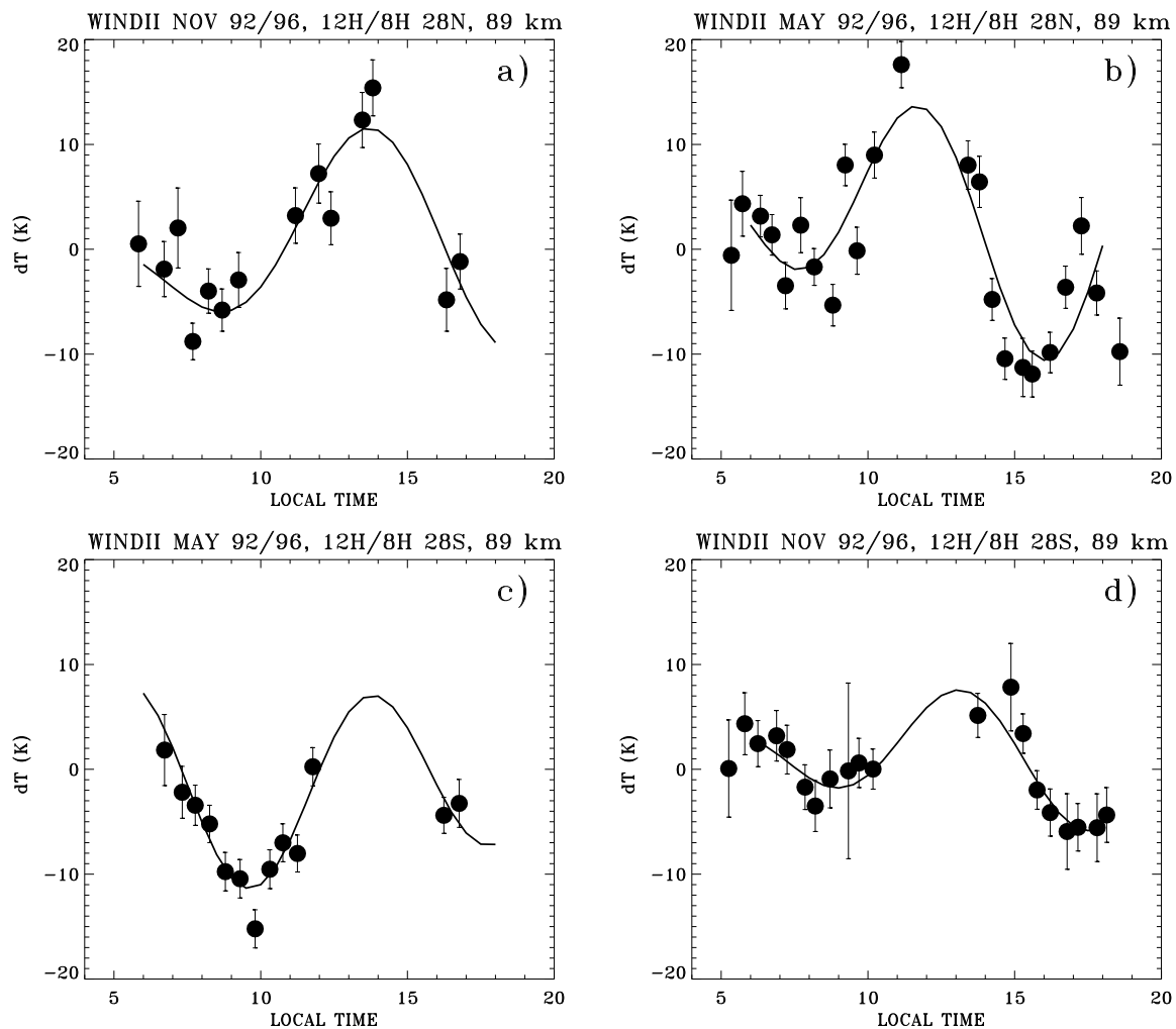
Fig. 3. WINDII temperature semidiurnal and terdiurnal tidal fits at 28^{\circ} N (a), (b) and 28^{\circ} S (c), (d) for the months of November and May. The temperature data are composites of observations from 1992 to 1996.
