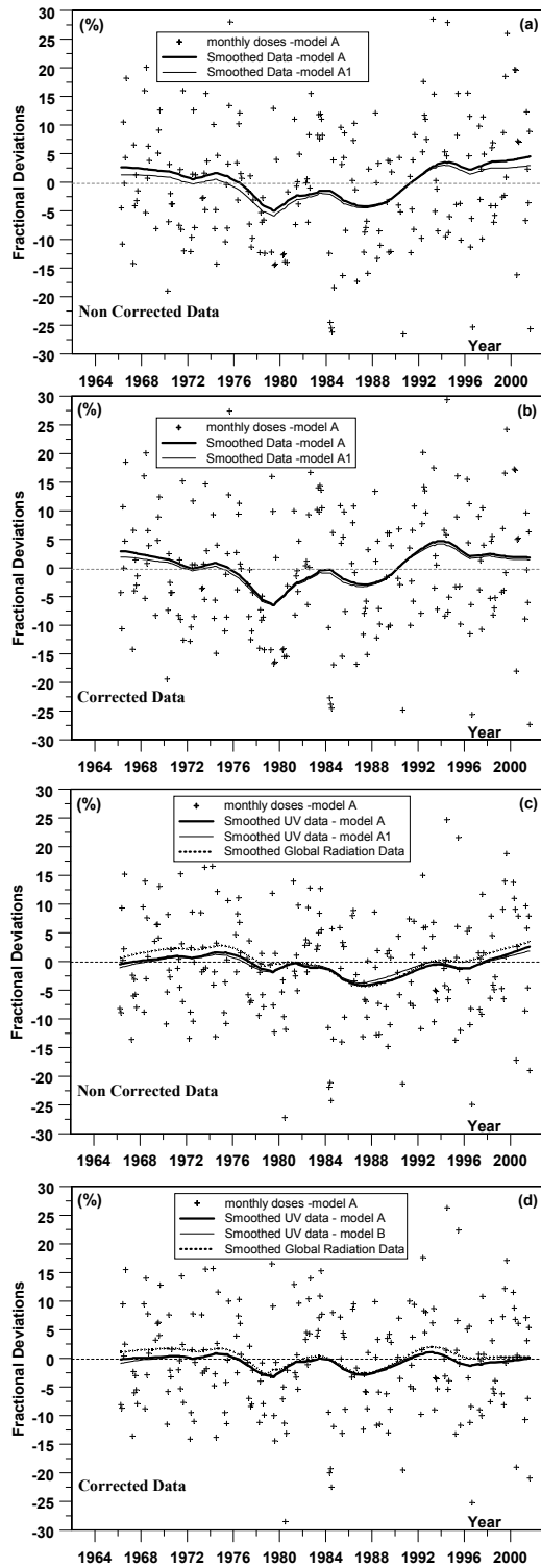
Fig. 5. The reconstructed monthly means (by model A) of UV fractional deviations and their smoothed pattern (by model A and A1); for non-corrected data set (a) and corrected data set (b) for Belsk. The cloud induced part of the reconstructed UV fractional deviations for non-corrected (c) and corrected (d) data set superposed on the monthly fractional deviations of measured total solar radiation. Curves represent smoothing by LOWESS.
