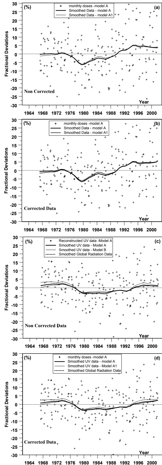
Fig. 7. The same as Fig. 5 but for Tõravere.
