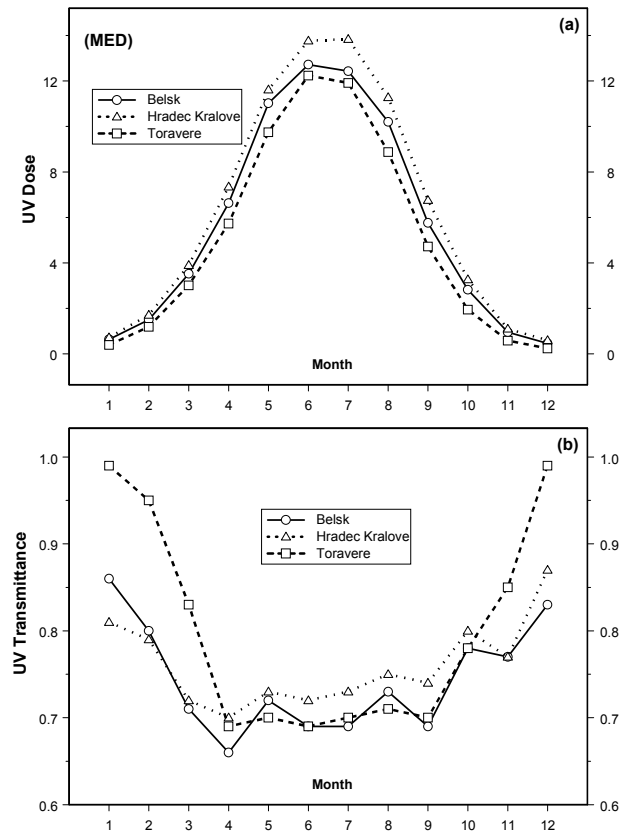
Fig. 4. The reconstructed seasonal pattern of the monthly mean dose (in MED unit) for Belsk, Hradec Kralove and Toravere (a), and the cloud reduction factor over these stations (b) for the period 1967–2001.
