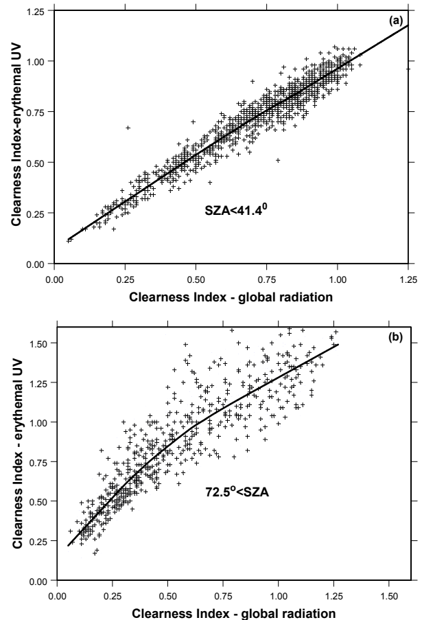
Fig. 2. The clearness index for UV radiation versus that for total solar radiation for the noon values of SZA < 41.4^\circ (a) and SZA > 72.5^\circ (b) Solid curve represents the cloud reduction factors (CRF) used in model A (see text).
