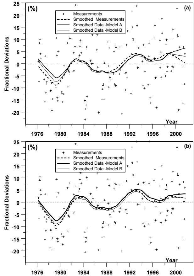
Fig. 3. The comparison between the modelled (model A and B) and observed monthly fractional deviations from the UV measurements carried out at Belsk in the April-September part of the year in the period 1976–2001. The measured monthly fractional deviations are superposed on the data smoothed by LOWESS; non-corrected data (a), corrected data (b).
