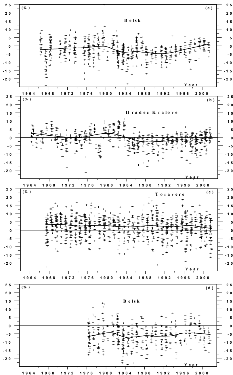
Fig. 1. The differences between measured and modelled daily sums of total solar radiation in percent of the modelled values for clear-sky conditions during the period April–September for Belsk (1966–2001) (a), Hradec Kralove (1964–2001) (b), and Tõravere (1967–2001) (c). The differences between measured and modelled daily doses in percent of the modelled values for clear-sky conditions over Belsk (1976–2001) (d). The solid curves represent the differences after a smoothing by the LOWESS technique.
