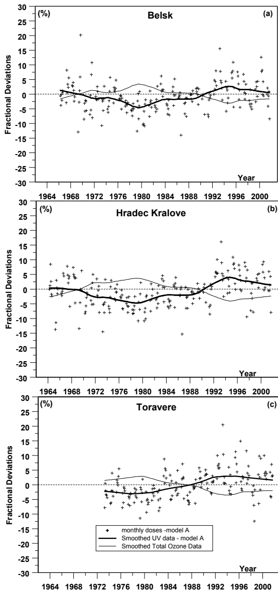
Fig. 8. The reconstructed (model A) monthly means of the total ozone induced part of the UV fractional deviations and their smoothed pattern (using LOWESS) for corrected data superposed on the monthly fractional deviations of measured total ozone over Belsk (a), Hradec Kralove (b), and Töravere (c).
