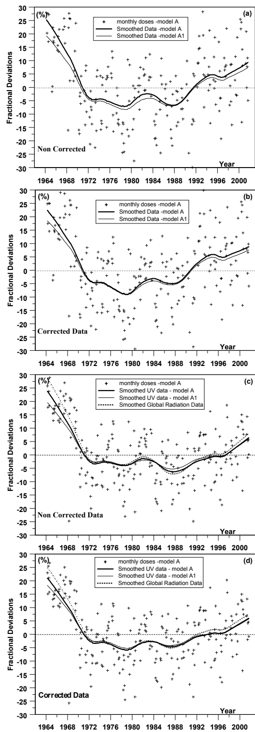
Fig. 6. The same as Fig. 5 but for Hradec Kralove.
