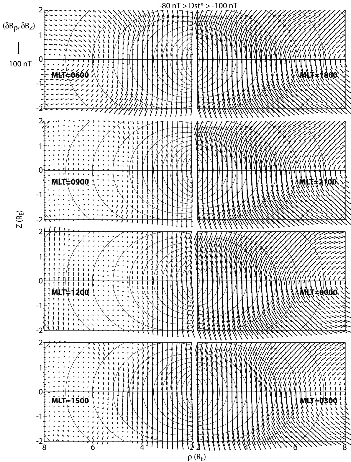
Fig. 4d. Meridional projection of the perturbation magnetic field arrows at equally spaced grids with superimposed dipole field lines in the meridian plane in each of the 8 magnetic local time bins and for each of the four D_{st}^* range: (d) -80 \text{ nT} > D_{st}^* > -100 \text{ nT} .
