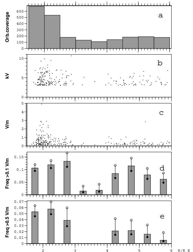
Fig. 7. Same as Fig. 6 but only potential minima deeper than 3 kV are included.
