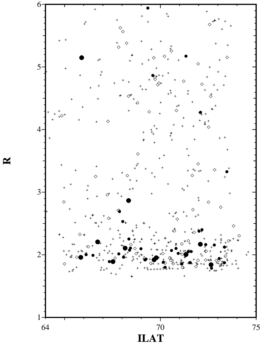
Fig. 5. Distribution of the minima against ILAT and R for the nightside (18:00–06:00 MLT) events. For details of the symbols, see caption of Fig. 4.
