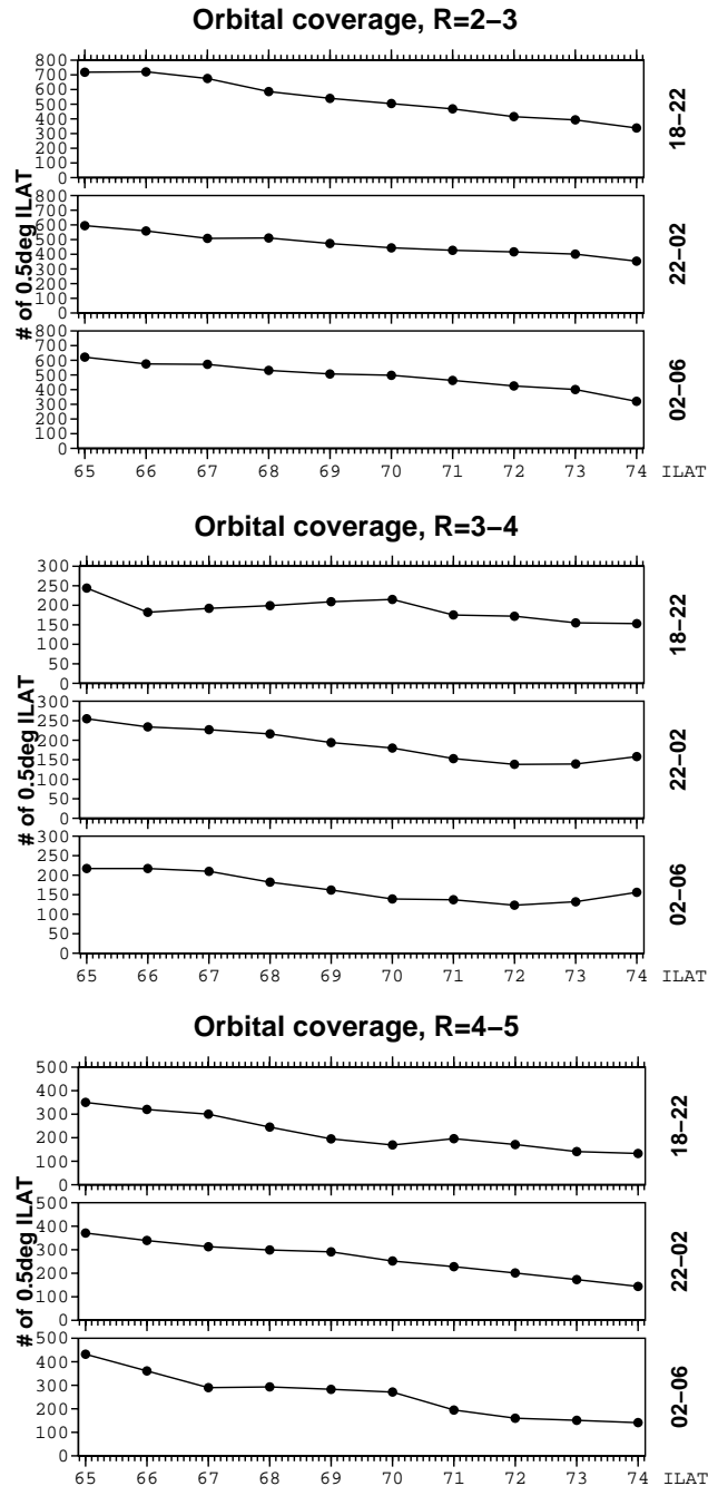
Fig. 16. Orbital coverage of Polar sectors satisfying our criteria of enough perpendicular trajectory in three radial distance ranges and in the three nightside MLT sectors.
