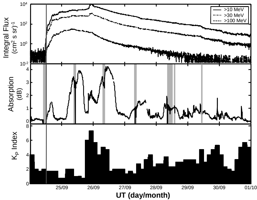
Fig. 3. Example of a PCA event from September 2001, in the same format as Fig. 2. Note the increase in K_p late on 25 September when a CME impacted the magnetosphere; this is reflected in the absorption data as a sharp rise shortly before midnight. At the same time the lower two energy channels from GOES-8 display increases in flux as the interplanetary shock accelerates the protons. Note that the absorption is more variable during this event, plus there are negative spikes and bays around local noon on each day.
