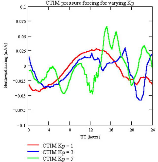
Fig. 9. The pressure gradient acceleration through the day for the same K_p levels as in Fig. 7.
