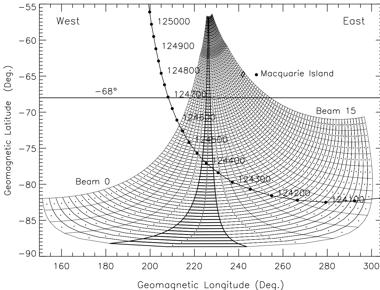
Fig. 2. The track of the DMSP F14 spacecraft through the TIGER field-of-view during 12:40:00 to 12:51:00 UT, 10 December 1999. The satellite track and the 75 range cells sampled on each of the 16 beams of TIGER have been plotted on the same grid of magnetic latitude and longitude. Beam 0 is the western-most beam (left) and beam 15 is the eastern-most beam (right). Beam 4, drawn in bold, points along the 226^{\circ} E magnetic meridian, but diverges towards the west at higher latitude. Range cell 26 of beam 15 is also drawn in bold because it is the closest observation cell to MQI on the same L-shell.
