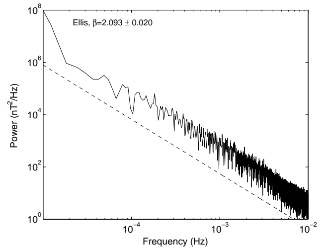
Fig. 3. Power spectra of magnetic data measured during 13–18 January 1993 at Ellisras (Ellis). The best-fit line gives a value for the spectral exponent of \beta = 2.093 \pm 0.020 . This line (dashed) is shifted for the purposes of comparison.
