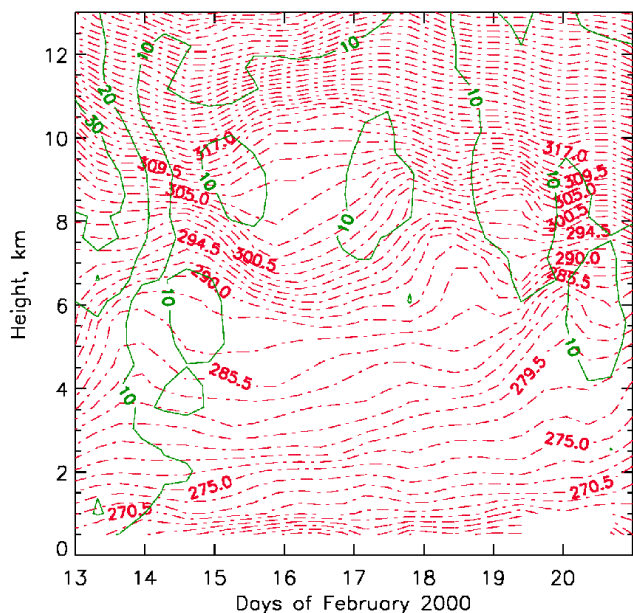
Fig. 4. Time series of potential temperature (red) and wind speed (green) at Sodankylä.
