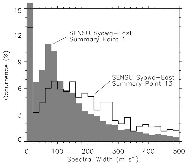
Fig. 7. The histogram of the spectral width distribution at S1 (shaded) and S13 (black line) in Syowa-East.
