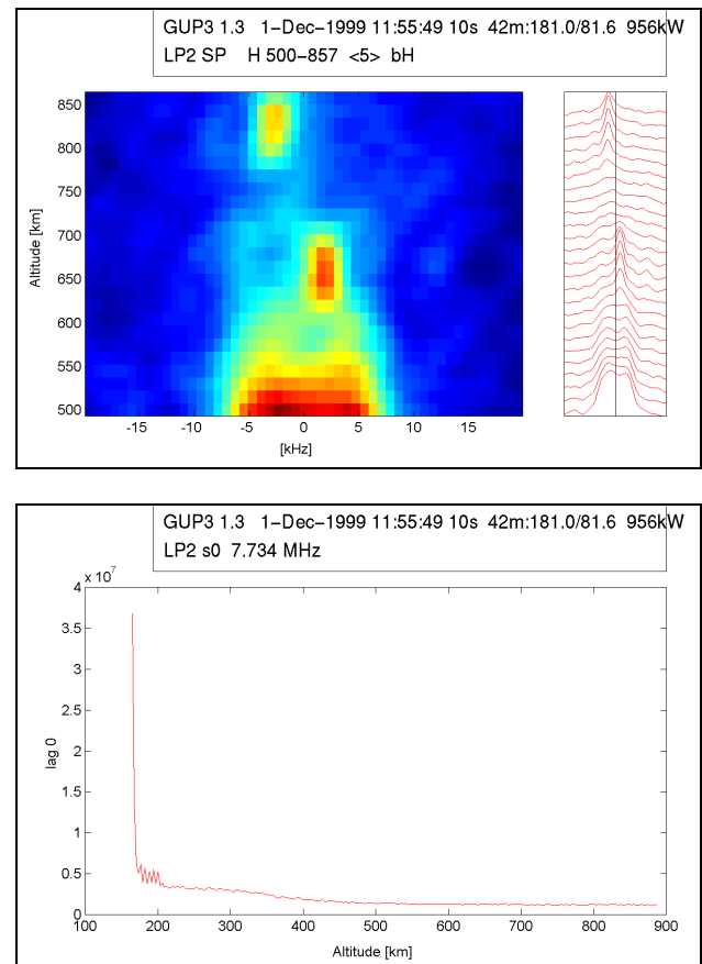
Fig. 2. Results showing (a) spectra, and (b) power profile for LP2 data at 11:55:49 UT, 1 December 1999, using EISCAT rtg3 program when enhanced spectra probably due to geophysical causes were seen in the beam.
