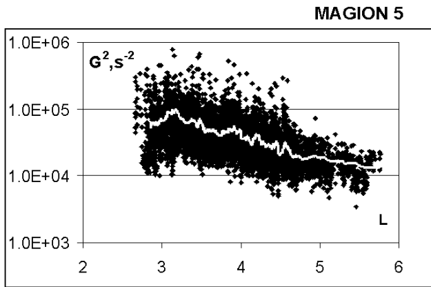
Fig. 6. The reduced sweep rate G^2 as a function of L-shell. The solid line shows the running average over 100 points of G^2 . The mean G(L) varies within a small interval 100–300 s -1 .
