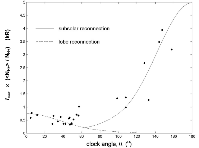
Fig. 10. Scatter plot of the normalised peak Lyman- \alpha emission intensity, I_{\max}\{\langle N_{H^+} \rangle / N_{H^+}\} , where N_{H^+} is the proton data seen by ACE and \langle N_{H^+} \rangle is its average value over the interval 15:00–16:00. The normalised intensities are averaged over 12:00–12:30 MLT and are plotted against the IMF clock angle in GSM observed by ACE, \theta (points). The ACE data have been lagged by the derived ACE-to-Earth propagation delay \delta t_E . The solid line shows the variation predicted by the cusp model for a subsolar reconnection site, the dashed line is the variation predicted for the same model inputs and a lobe reconnection site.
