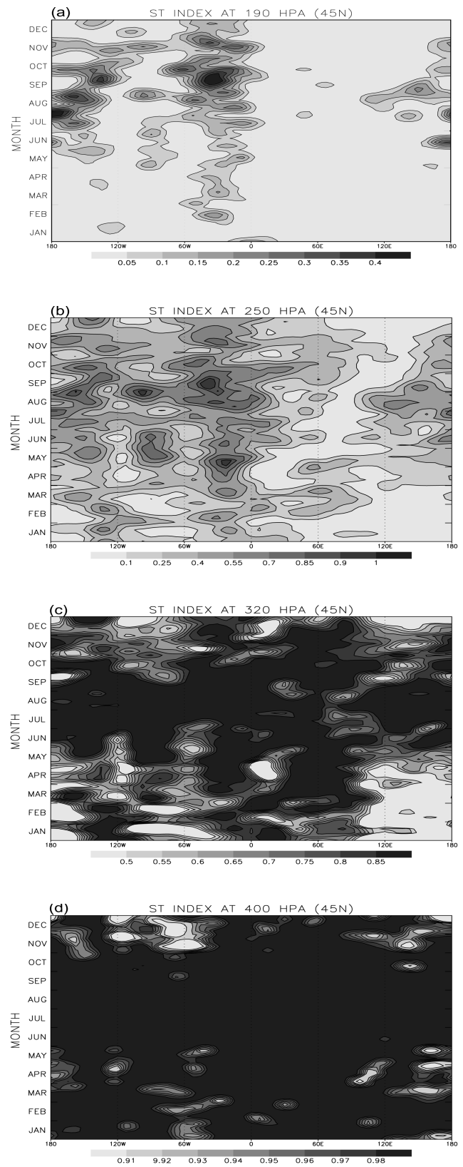
Fig. 3. The same as in Fig. 2 but for latitude at 45° N.
