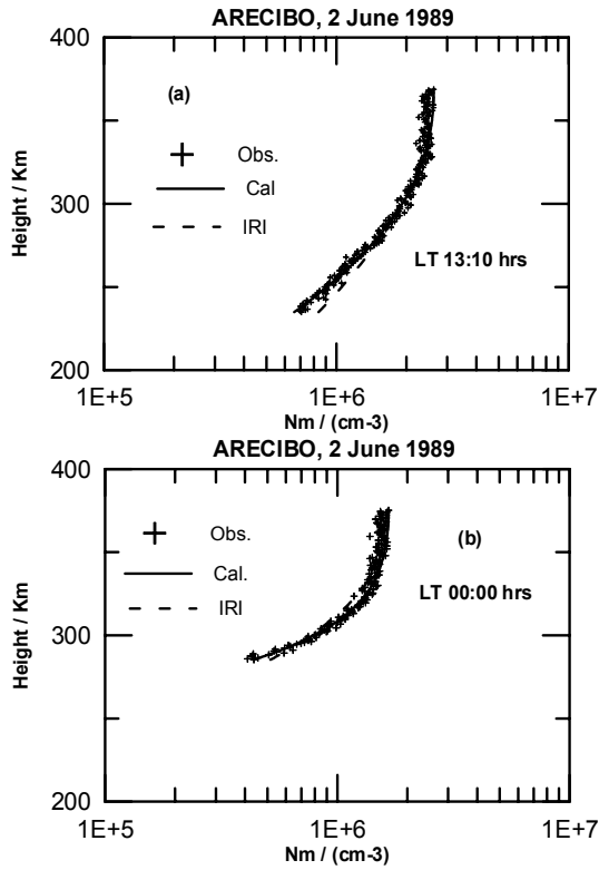
Fig. 1. Sample profiles obtained using best B_0 , B_1 parameters derived from I.S. measurements at Arecibo for (a) daytime, (b) mid-night. Calculated profiles are shown by solid lines. The IRI model profile is shown as dash line.
