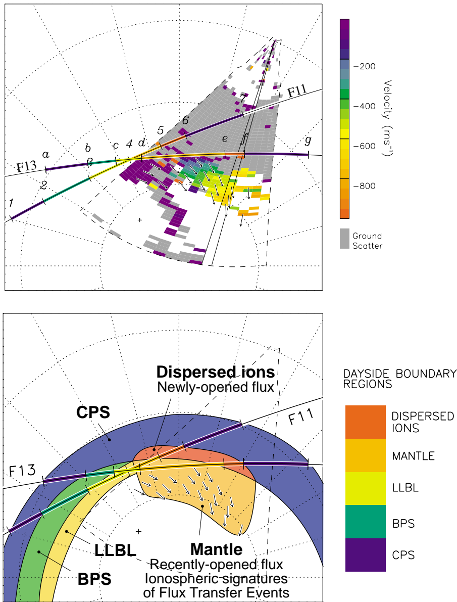
Fig. 3. (a) Polar plot of the l-o-s velocity as observed by all the beams of the Hankasalmi radar at 08:04 UT. The plot is in a geomagnetic/MLT coordinate system, and the radar is pointing towards local noon. Beam 4 is marked with a black line. Beam-swinging vectors are overlaid on the plot. Also overlaid are the tracks of the F11 and F13 spacecraft for the time interval shown in Fig. 2. Indicated on the tracks are the dayside boundary regions as defined from the ion and electron spectrograms. (b) A schematic illustration of the results presented in Fig. 3a. The diagram presents the tracks of the F11 and F13 spacecraft, and the different dayside boundary regions. The field of view of the Hankasalmi radars and the derived beam-swinging vectors are also shown on the plot.
