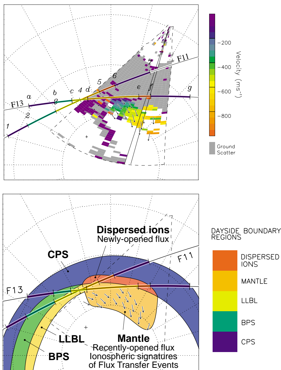
Fig. 3. (a) Polar plot of the l-o-s velocity as observed by all the beams of the Hanksalmi radar at 08:04 UT. The plot is in a geomagnetic/MLT coordinate system, and the radar is pointing towards local noon. Beam 4 is marked with a black line. Beam-swinging vectors are overlaid on the plot. Also overlaid are the tracks of the F11 and F13 spacecraft for the time interval shown in Fig. 2. Indicated on the tracks are the dayside boundary regions as defined from the ion and electron spectrograms. (b) A schematic illustration of the results presented in Fig. 3a. The diagram presents the tracks of the F11 and F13 spacecraft, and the different dayside boundary regions. The field of view of the Hanksalmi radars and the derived beam-swinging vectors are also shown on the plot.
