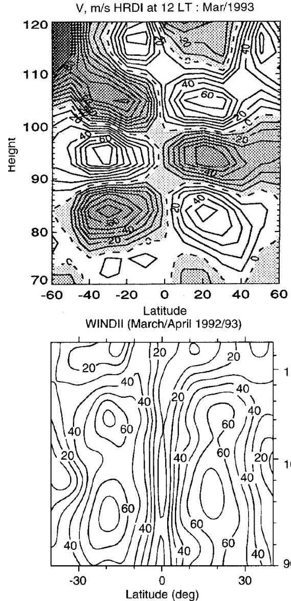
Fig. 5. Meridional winds ( \text{ms}^{-1} ) at 12:00 LT for March, as measured by HRDI (top) (from Yudin et al., 1997), with southward winds shaded, and the diurnal amplitude structure of meridional winds ( \text{ms}^{-1} ) as measured by WINDII (bottom) (from Akmaev et al., 1997).
