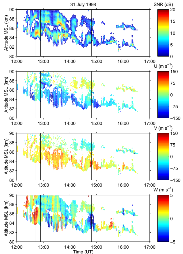
Fig. 1. Range-time pseudocolor plots of the signal-to-noise ratio (SNR); zonal (U) and meridional (V) components of the horizontal wind; and the vertical velocity (W). The black vertical lines are used to flag times that have been selected for closer examination.
