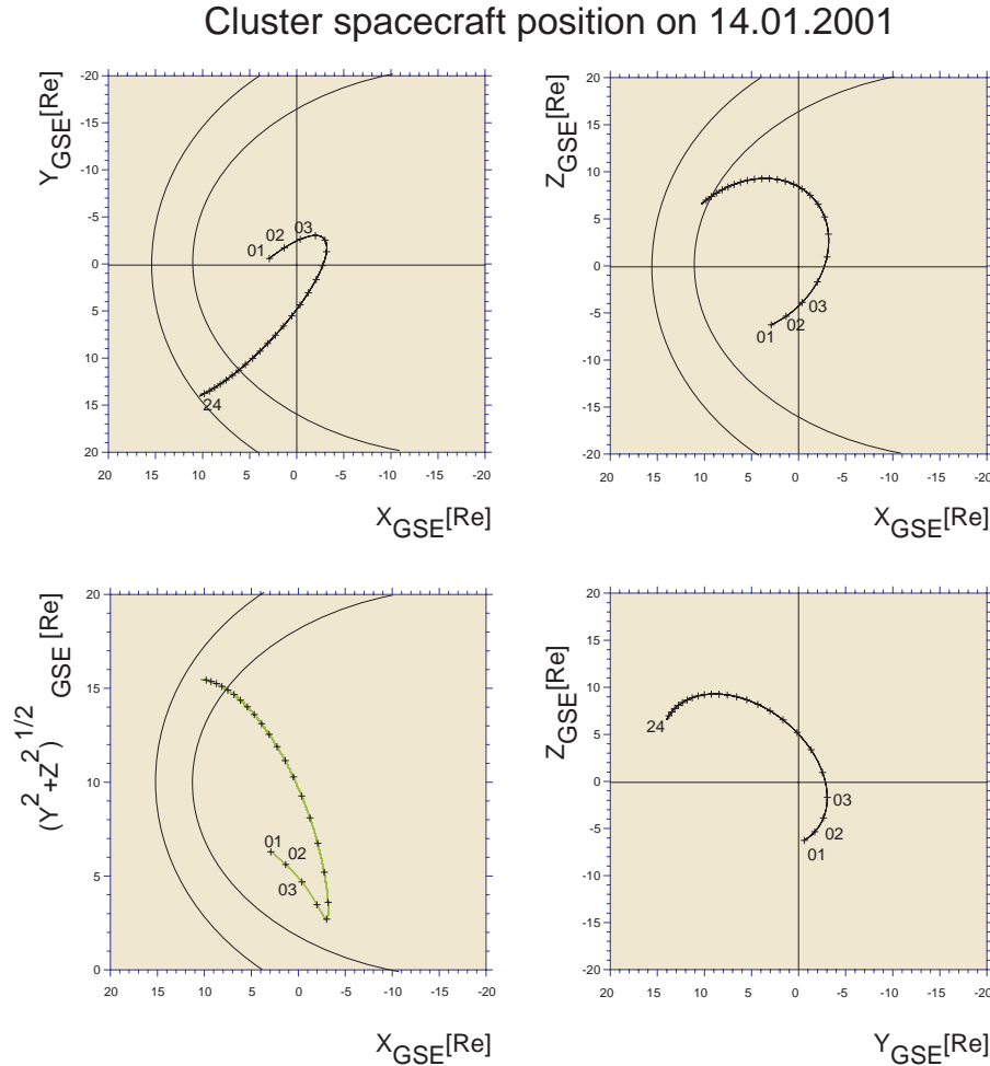
Fig. 3. The orbit of the Cluster fleet on 14 January 2001. The tick marks denote the spacecraft position in intervals of one hour.
