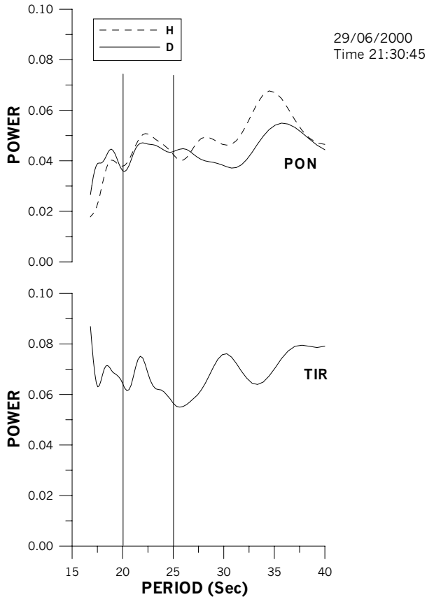
Fig. 9. The lower panel shows the power spectrum of 5 s averaged filter scintillations at Tirunalvely on the specified day and at local time. The dashed and solid curves in the upper panel respectively, show the power spectrum of H- and D-variations of ground magnetic data of 5 s sampling interval at Pondicherry. The range of the eigen-period has been marked by the interval between two vertical lines.
