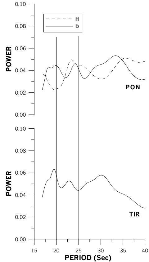
Fig. 10. The lower panel shows the power spectrum of 5 s averaged filter scintillations at Tirunalvely on the specified day and at local time. The dashed and solid curves in the upper panel, respectively, show the power spectrum of H- and D-variations of ground magnetic data of 5 s sampling interval at Pondicherry. The range of the eigen-period has been marked by the interval between two vertical lines.
