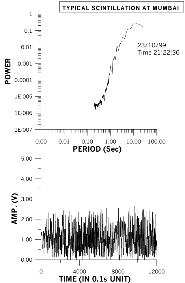
Fig. 2. The lower panel shows a typical scintillation at Mumbai, and the upper panel displays the corresponding power spectrum showing that field line eigen-period ( \sim 25 sec) falls well beyond the Fresnel zone.
