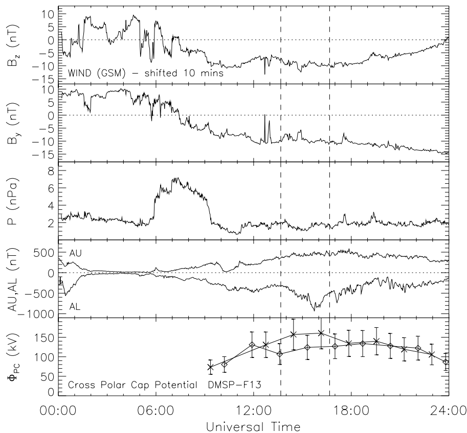
Fig. 2. Data presenting an overview of solar wind and magnetospheric variations on 20 August 1998. The panels show the interplanetary magnetic field B_z and B_y components (in GSM coordinates) and solar wind dynamic pressure from the WIND spacecraft, the AU and AL index variations, and the cross-polar cap potential estimate from DMSP-F13.
