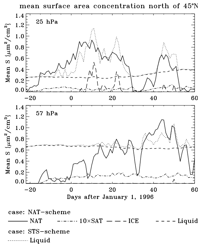
Fig. 3. Temporal change of particle surface area concentrations ( \mu\text{m}^2 \text{ cm}^{-3} ) averaged over the area north of 45° N on the model levels (bottom frame) 57 hPa and (top frame) 25 hPa. Data is presented for the time period between 10 December 1995, and 29 February 1996, simulated in the model experiments performed with the NAT- and the STS-scheme, respectively.
