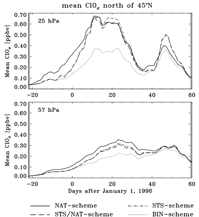
Fig. 6. Temporal change of the ClO x (:=Cl + ClO + 2 Cl 2 O 2 +2 Cl 2 +HOCl+OCIO) mixing ratio (ppbv) averaged over the area north of 45° N on the model levels (bottom frame) 57 hPa and (top frame) 25 hPa. Results are presented for the time period between 10 December 1995, and 29 February 1996, simulated in the model experiments performed with the NAT-, the STS-, the STS/NAT- and the BIN-scheme, respectively.
