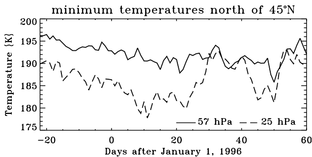
Fig. 2. Temporal change of model minimum temperatures within the area north of 45° N. Data is presented for the time period between 10 December 1995, and 29 February 1996, and the model levels 57 and 25 hPa.
