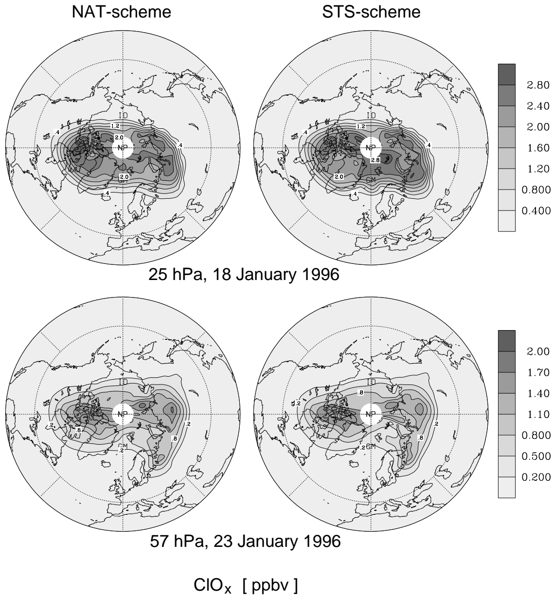
Fig. 7. \text{ClO}_x ( :=\text{Cl}+\text{ClO}+2\text{Cl}_2\text{O}_2+2\text{Cl}_2+\text{HOCl}+\text{OCIO} ) mixing ratio (ppbv) modelled for (top frames) the 25 hPa and (bottom frames) the 57 hPa levels. Results are shown for two selected days of January 1996 showing comparatively large chlorine activation (57 hPa level on 23 January 1996, and 25 hPa level on 18 January 1996). The left frames and right frames show data modelled applying the NAT- and the STS-scheme, respectively.
