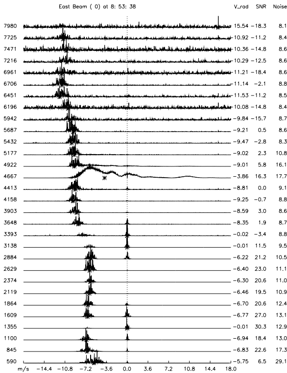
Fig. 3. The left part shows the “stacked spectrum” plot, i.e. the Doppler spectra for each range gate, for the radar dwell at 08:53:38 UTC on 1 December 1999. The right figures give a detailed look into the raw data (I/Q-timeseries) and the Doppler spectrum for the gates 11 and 17 (whose data will be wavelet processed). The black arrows indicate the estimated first moment (i.e. the radial velocity).
