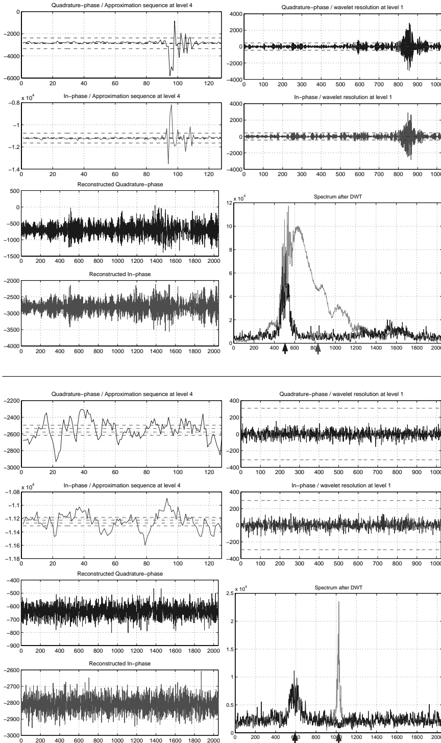
Fig. 7. Decomposition ( \alpha_k und \beta_{1k} ), reconstruction and Fourier power spectrum of gate 17 (top) and gate 11 (below). The black curves in the power spectra representations display the decontaminated spectra. One clearly recognizes the differences of moment estimations; see the computed first moment before (gray arrow) and after (black arrow) the filtering step.
