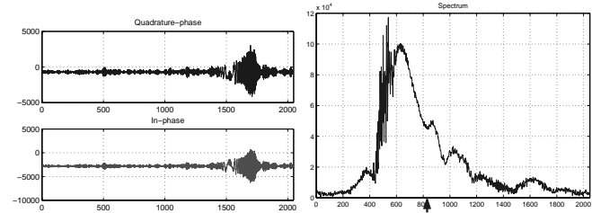
Raw data (I/Q-time series) of gate 17 and the resulting power spectrum
