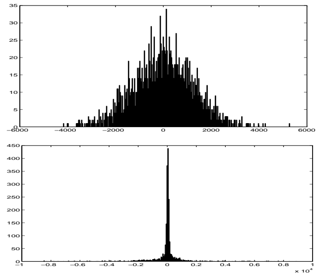
Fig. 6. This figure shows typical histograms of the wavelet coefficients (see text). The upper histogram represents an in-phase series without an airplane echo and the lower histogram represents an in-phase series with an airplane reflection.
