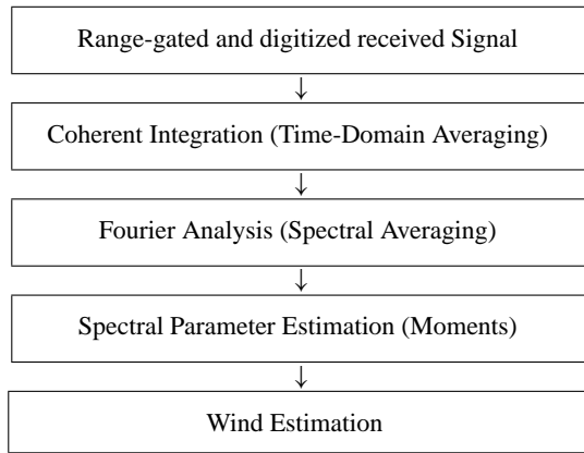
Fig. 1. The figure shows the flow diagram of 'classical' digital signal processing.
