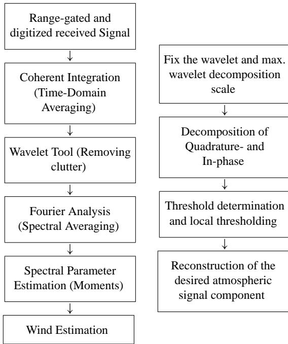
Fig. 5. Left: The flow diagram extended by the wavelet tool. Right: The wavelet algorithm flow diagram.
