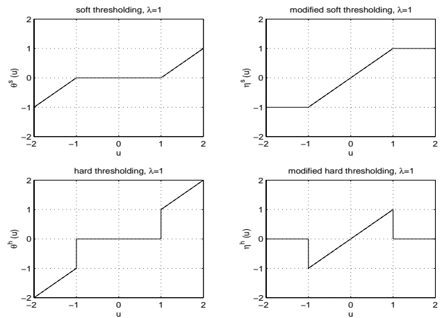
Fig. 4. This figure shows hard and soft thresholding.
