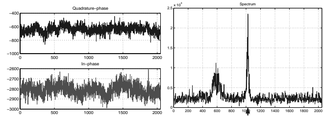
Raw data (I/Q-timeseries) of gate 11 and the resulting power spectrum
