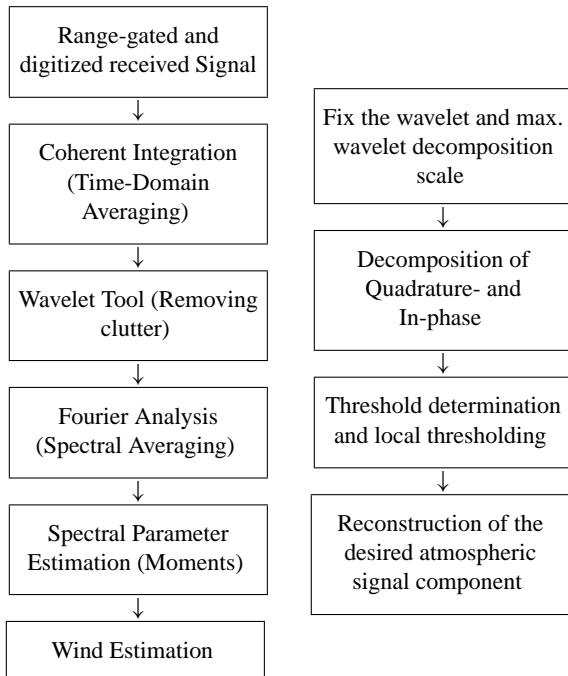
Fig. 5. Left: The flow diagram extended by the wavelet tool. Right: The wavelet algorithm flow diagram.
