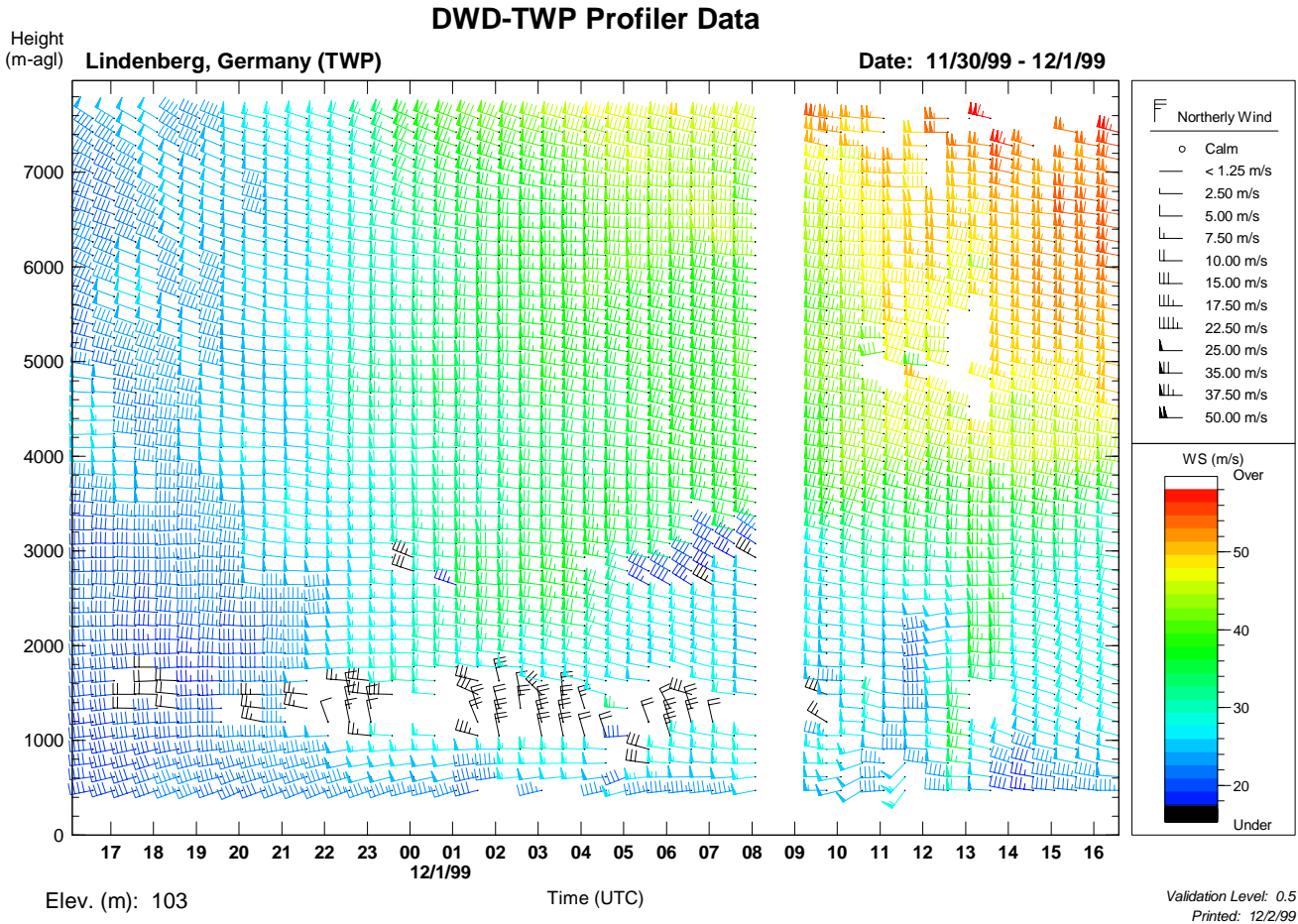
Fig. 2. The figure shows the final result of the measurement with the 482 MHz RWP at Lindenberg (Germany) on the 30 November and 1 December 1999. The wind barbs are color-coded according to the wind speed. Note the effects of the persistent ground clutter around the 1500 m and 3000 m heights. The gap in the data was caused by this detailed investigation, as the radar was programmed to store time series data for about 30 minutes, only in the East beam, thus, no wind computations were possible for that period of time.
