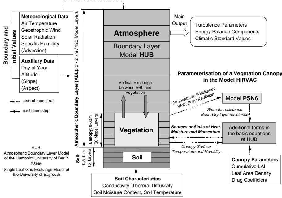
Fig. 1. Scheme of the model HIRVAC.
