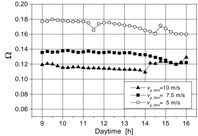
Fig. 3. Dependence of the decoupling coefficient \Omega on geostrophic wind speed; simulation with the model HIRVAC for 3 July and clear sky ( h_{veg} = 27.5 m, n_w = 0.8 , LAI = 5 ).
