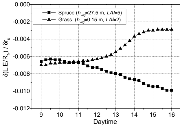
Fig. 6. Sensitivity of the evaporative fraction to canopy resistance dependent on the type and height of vegetation; simulation with the model HIRVAC for 3 July and clear sky.
