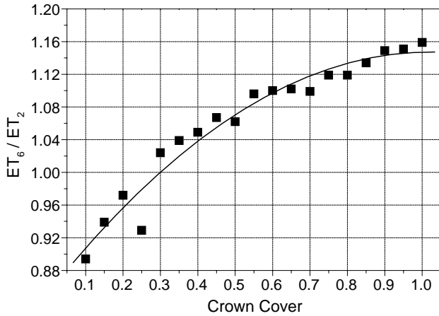
Fig. 4. Relation in daily sum of evapotranspiration between model days 6 and 2; dependence on crown cover; simulation with the model HIRVAC for 21 June, clear sky and a spruce stand ( h_{\text{veg}} = 27.5 m, LAI = 5 ).
