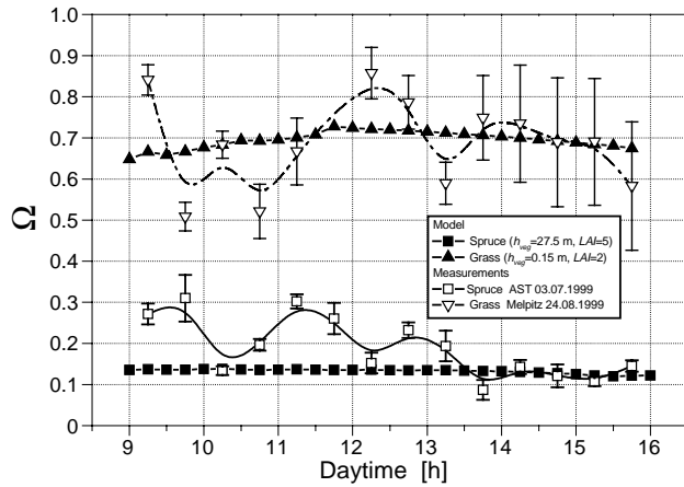
Fig. 2. Dependence of the decoupling coefficient \Omega on the type and height of vegetation; comparison of results from HIRVAC simulation with measurements from 3 July (spruce) and 24 August (grass) under clear sky conditions (error bars – standard deviation of 10-min-measurements).
