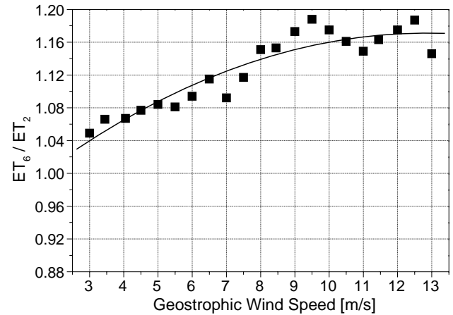
Fig. 5. Relation in daily sum of evapotranspiration between model days 6 and 2; dependence on geostrophic wind speed; simulation with the model HIRVAC for 21 June, clear sky and a spruce stand ( h_{\text{veg}} = 27.5 m, LAI = 5 ).
