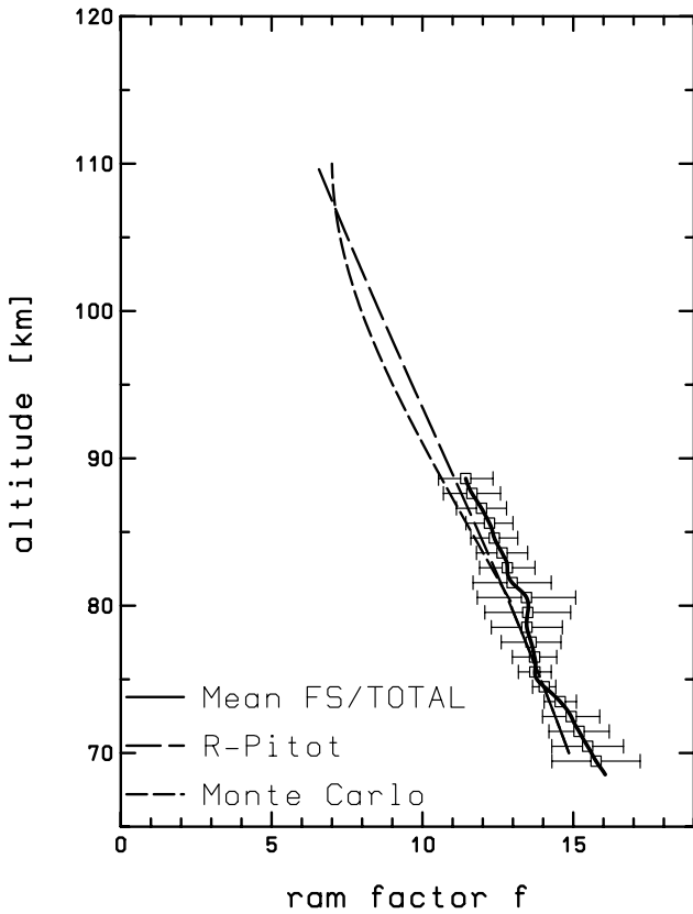
Fig. 7. Mean altitude profile of density ratios between TOTAL and falling sphere measurements (thick solid line). Error bars indicate the rms variation of the data. In addition, the results from the DSMC calculations (short dashed line) and a ram-factor calculated with the Rayleigh-Pitot formula (long dashed line) (Shapiro, 1954) are shown.
