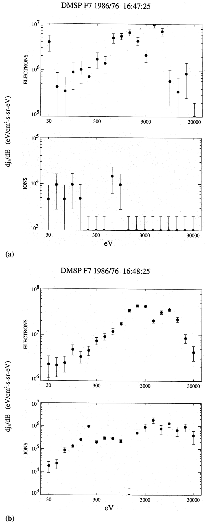
Fig. 3a-b. Electron and ion spectra observed at low altitude by DMSP F7 for the pass shown in Fig. 1. Plotted is the differential energy flux (circles with error bars) for various plasma regimes: (a) DAZ; (b) AO.
