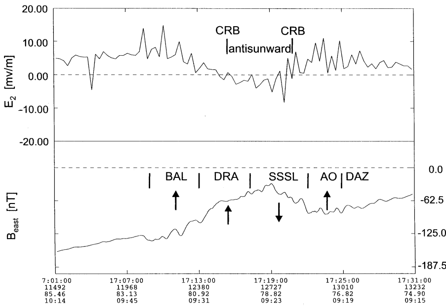
Fig. 7. The east-west component of the Viking magnetometer observations (bottom) and the spin plane component of the electric field (the component along the spacecraft trajectory, top) for the pass shown in Fig. 1: (a) the evening sector, (b) the pre-noon sector. The plasma regimes intersected by the satellite and directions of the FACs are marked at the top.
