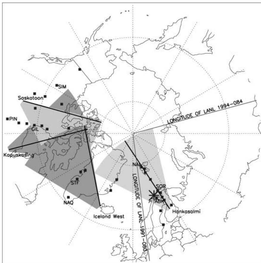
Fig. 1. Location of instruments. Magnetometer networks shown are MARIA in Canada, IMAGE in Scandinavia and DMI magnetometers on Greenland. The SuperDARN radars' field-of-view and EISCAT Tromsø (asterisk) are also displayed. Geostationary satellite positions are depicted by longitudinal lines
