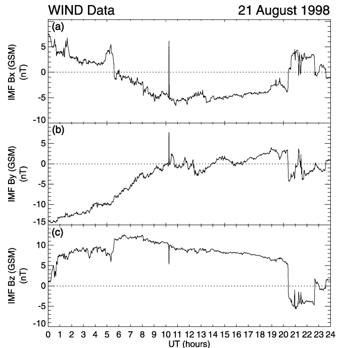
Fig. 2. Data from the Wind spacecraft upstream in the solar wind for the interval 0000–2400 UT on the 21st August, 1998. Panels a–c show the X , Y and Z component magnetic field data in GSM coordinates
