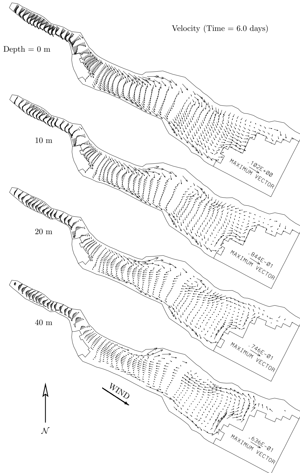
Fig. 10. Velocity vectors, 6 days after a constant northwest wind (305° NW in the longitudinal direction of the basin) started, in 0 m, 10 m, 20 m and 40 m depth. Each panel has its own velocity scale.
