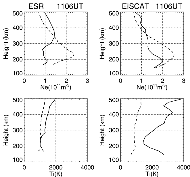
Fig. 4. Height profiles of N_e and T_i measured by ESR ( left ) and EISCAT ( right ) under both quiet ( dashed ) and disturbed ( solid ) conditions
