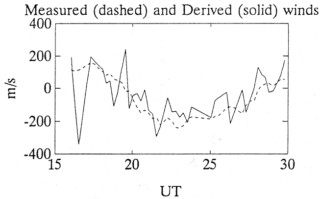
Fig. 8. Comparison of meridional winds directly measured by the FPI at Kiruna with those derived from EISCAT plasma velocities using the assumption of diffusive equilibrium. Data from the 21 st January 1990 show that under very particular conditions that may be tested statistically the derivation can be successful (from Davis, 1993).
