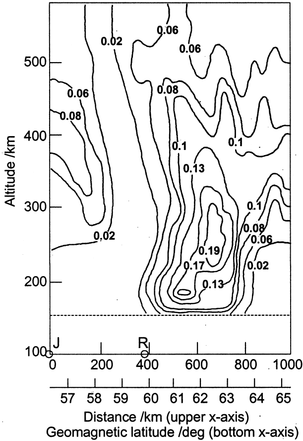
Fig. 3. Reconstructed image of the electron density ( \times 10^{12} \text{ m}^{-3} ) observed in the vertical plane over the tomographic chain in the USA and Canada in the evening at 00:41 UT on 4 November, 1993. The inversion is made by means of the phase difference tomographic method. The upper x-axis shows the distance on the ground (km), and the bottom axis indicates the geomagnetic latitude (degrees). The receiver sites from north to south are: Roberval, Canada ( 48.42^\circ \text{ N} , 385 km); Jay, VT ( 44.95^\circ \text{ N} , 0 km); Hanscom AFB, MA ( 42.45^\circ \text{ N} , -277 km), and Block Island, RI ( 41.17^\circ \text{ N} , -419 km). Only the most northern sites are shown by open dots on the horizontal axis.
